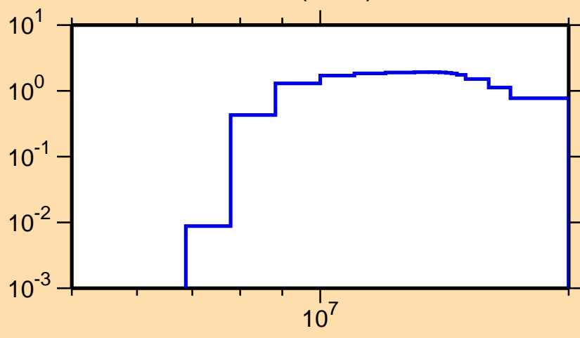
\sigma vs. E for ^{153}\text{Pm}(n,2n)
