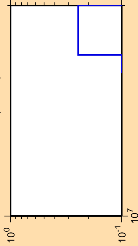
\Delta\sigma/\sigma vs. E for ^{153}\text{Pm}(n,3n\alpha)
