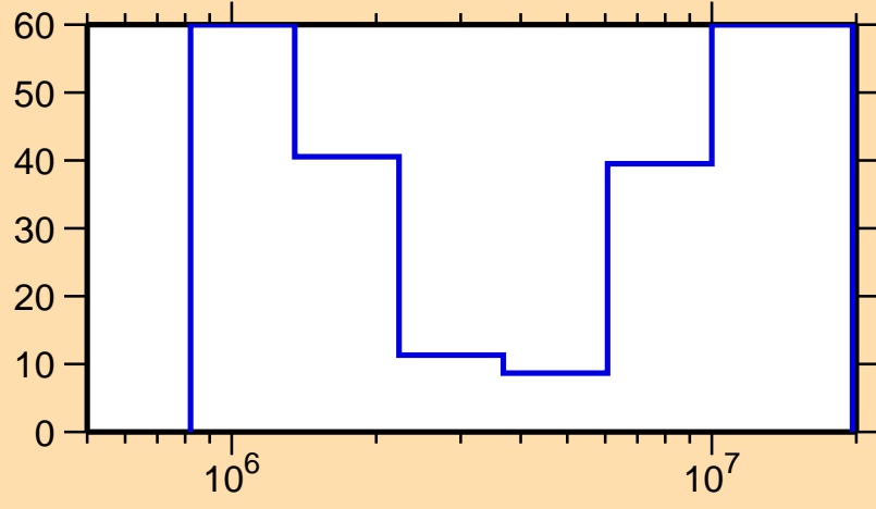
\Delta\sigma/\sigma vs. E for ^{153}\text{Pm}(n,n\text{cont.})
