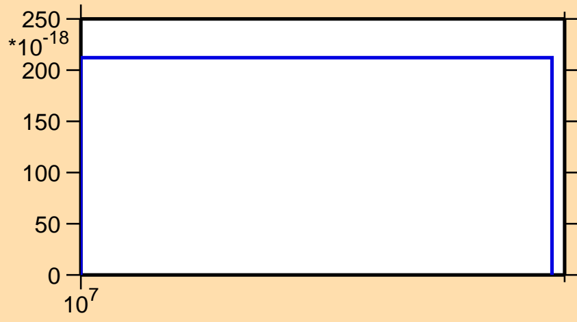
\sigma vs. E for ^{153}\text{Pm}(n,3n\alpha)
