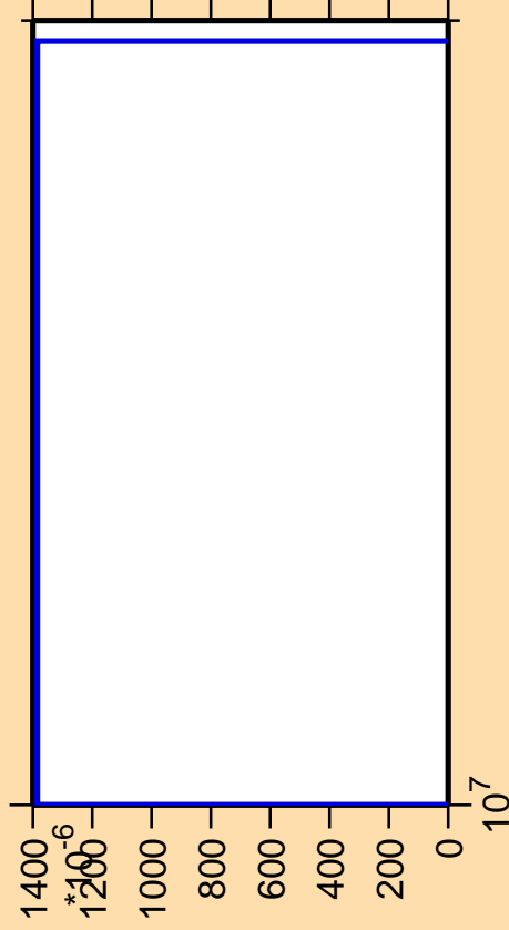
\Delta\sigma/\sigma vs. E for ^{153}\text{Pm}(n,3n\alpha)
