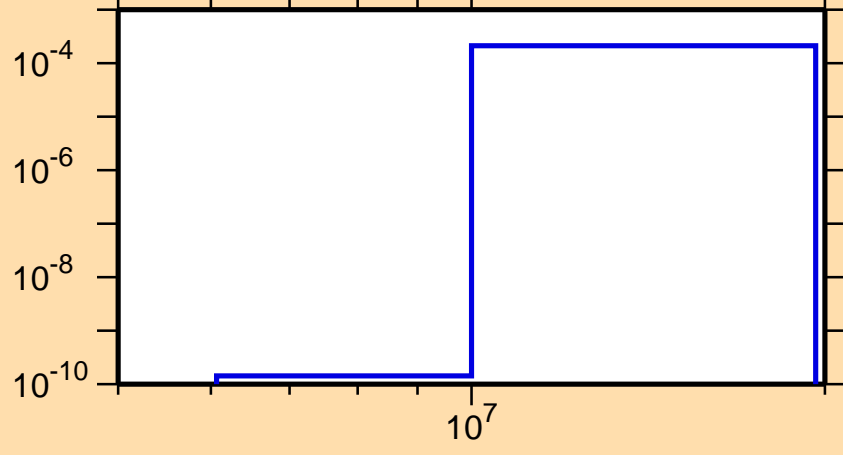
\sigma vs. E for ^{153}\text{Pm}(n,d)
