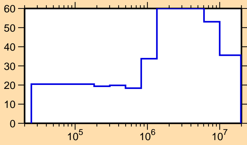
\Delta\sigma/\sigma vs. E for ^{153}\text{Pm}(n,n_1)
