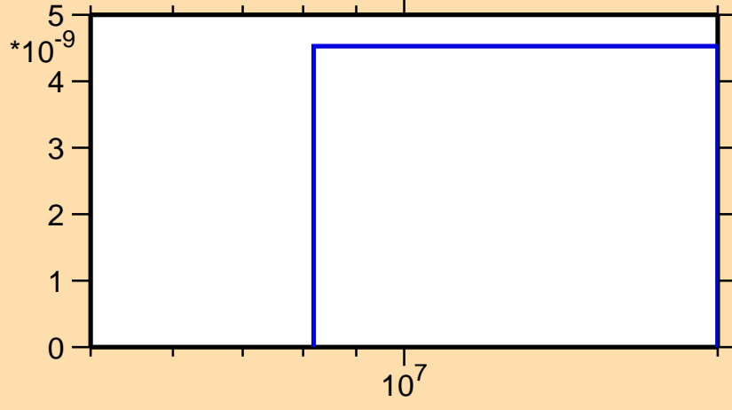
\sigma vs. E for ^{153}\text{Pm}(n,nd)
