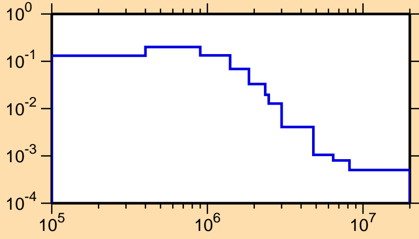
\sigma vs. E for ^{153}\text{Pm}(n,n_3)
