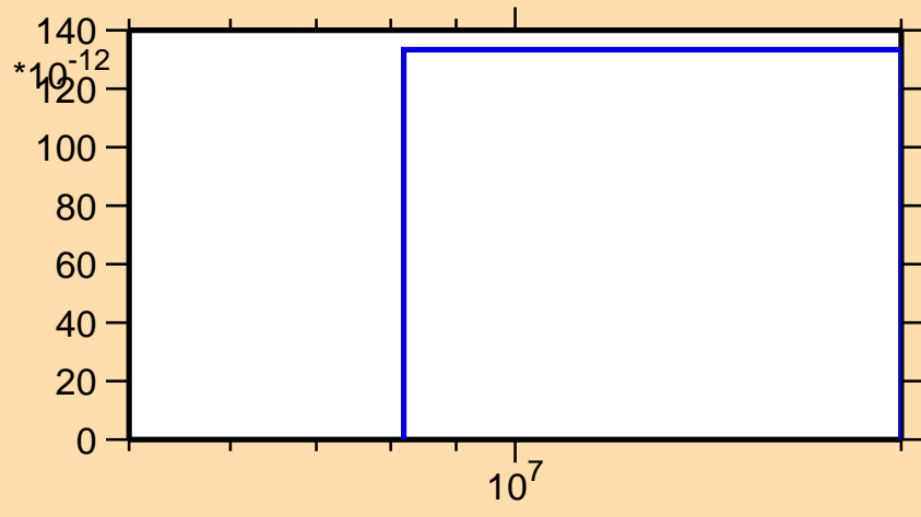
\sigma vs. E for ^{153}\text{Pm}(n,2np)
