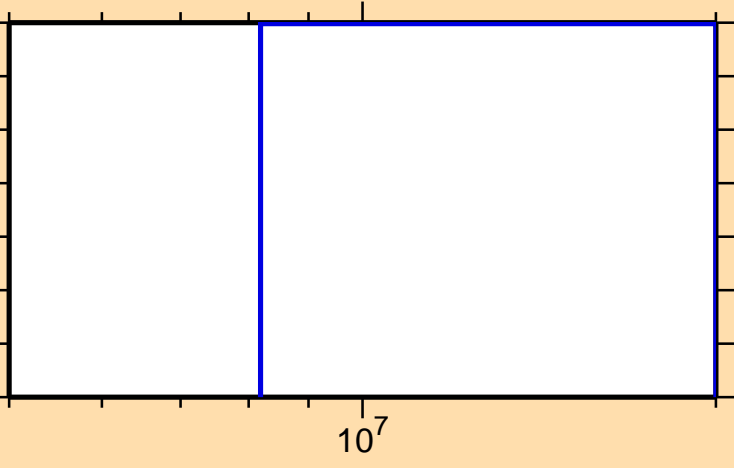
\sigma vs. E for ^{153}\text{Pm}(n,np)
