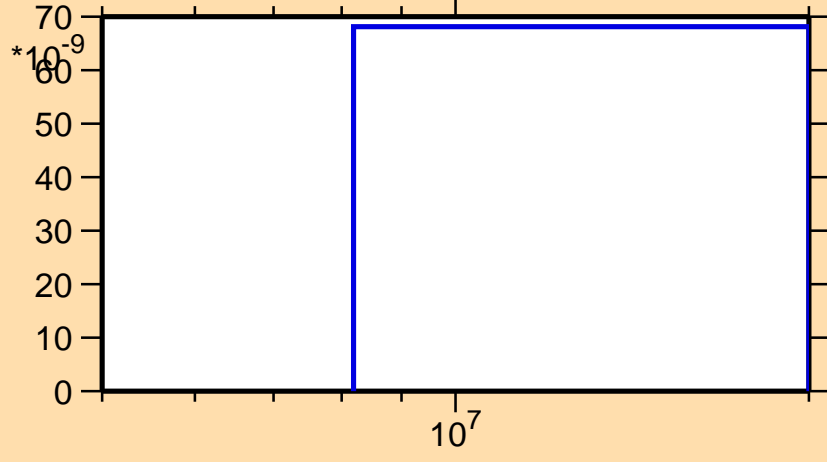
\sigma vs. E for ^{154}\text{Pm}(n,nd)
