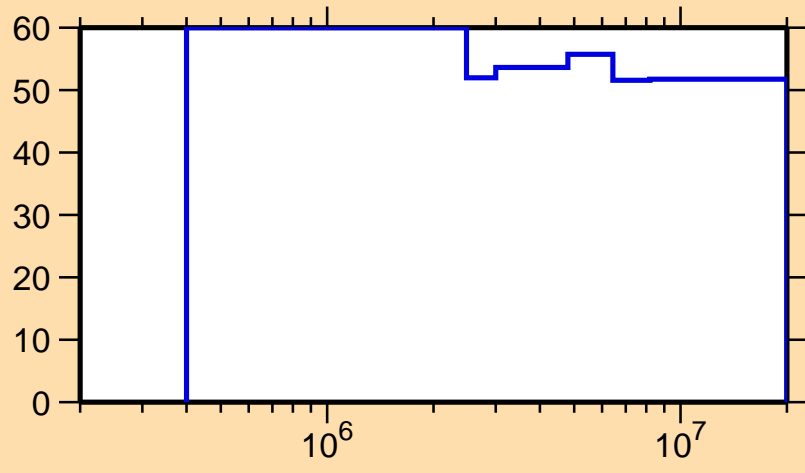
\Delta\sigma/\sigma vs. E for ^{154}\text{Pm}(n,n_1)
