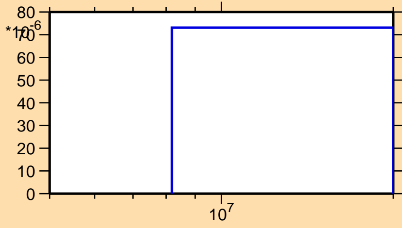
\sigma vs. E for ^{154}\text{Pm}(n,np)
