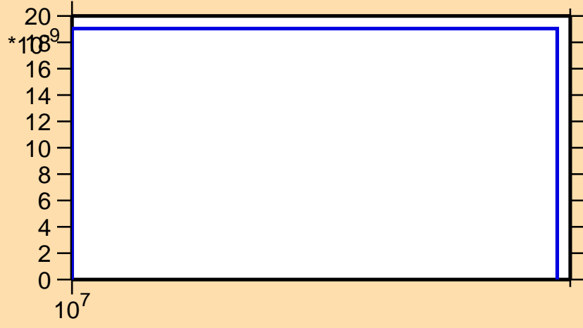
\sigma vs. E for ^{155}\text{Pm}(n,nt)
