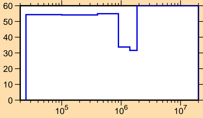
\Delta\sigma/\sigma vs. E for ^{155}\text{Pm}(n,n_1)
