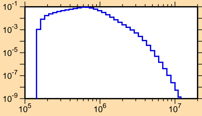
\sigma vs. E for ^{156}\text{Pm}(n,n_2)
