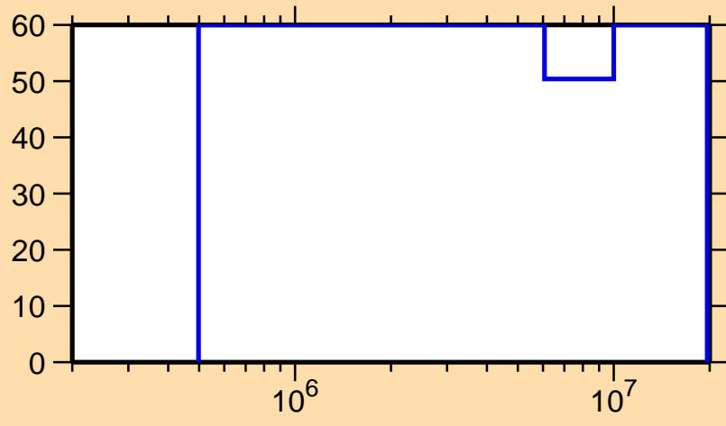
\Delta\sigma/\sigma vs. E for ^{156}\text{Pm}(n,n\text{cont.})
