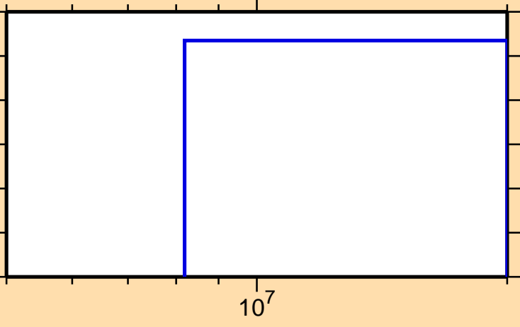
\sigma vs. E for ^{156}\text{Pm}(n,d)
