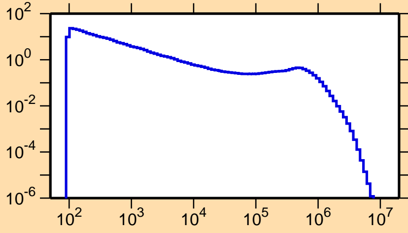
\sigma vs. E for ^{156}\text{Pm}(n,n_1)
