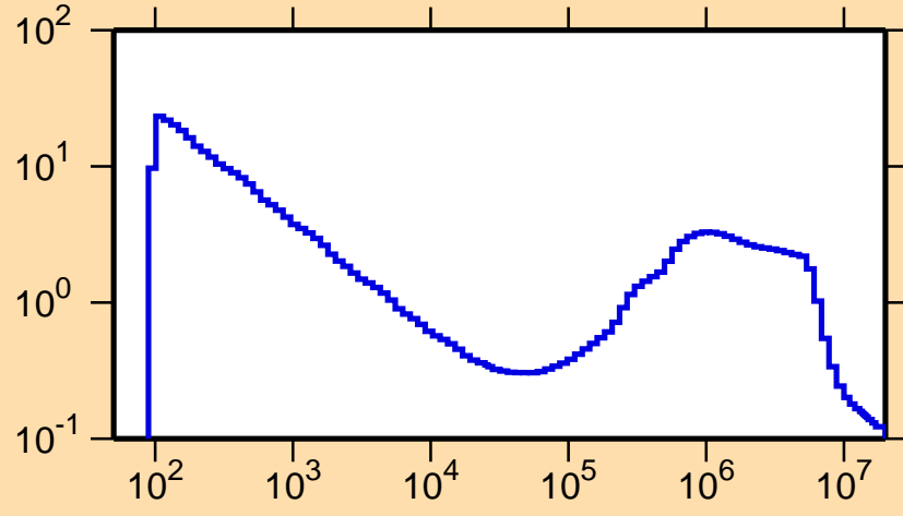
\sigma vs. E for ^{156}\text{Pm}(n,\text{inel.})
