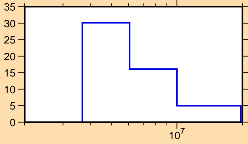
\Delta\sigma/\sigma vs. E for ^{156}\text{Pm}(n,el.)
