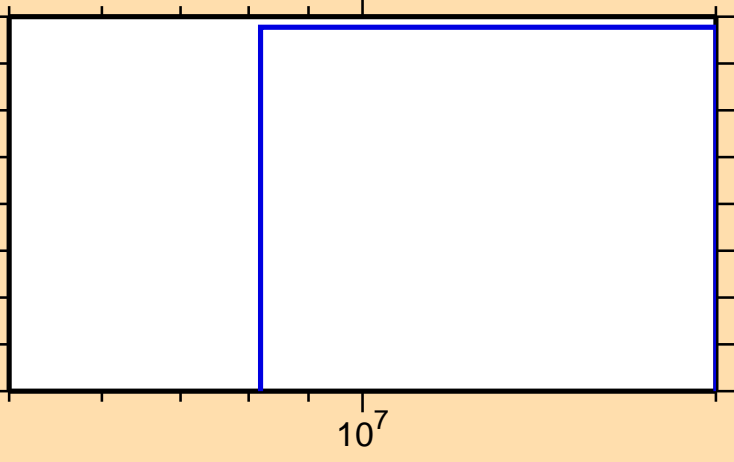
\sigma vs. E for ^{156}\text{Pm}(n,np)
