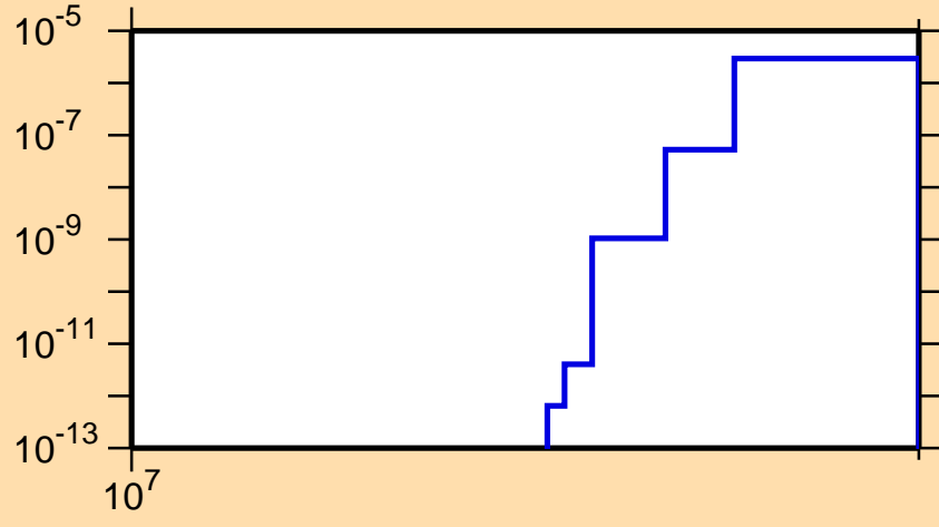
\sigma vs. E for ^{157}\text{Pm}(n,nt)
