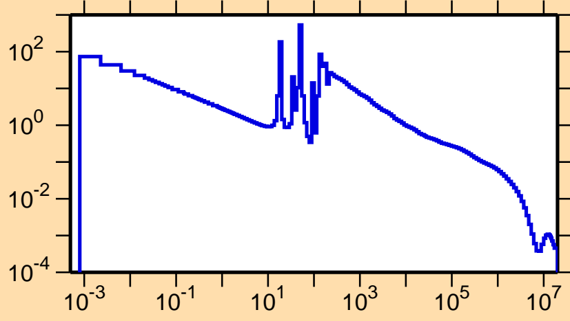
\sigma vs. E for ^{157}\text{Pm}(n,\gamma)
