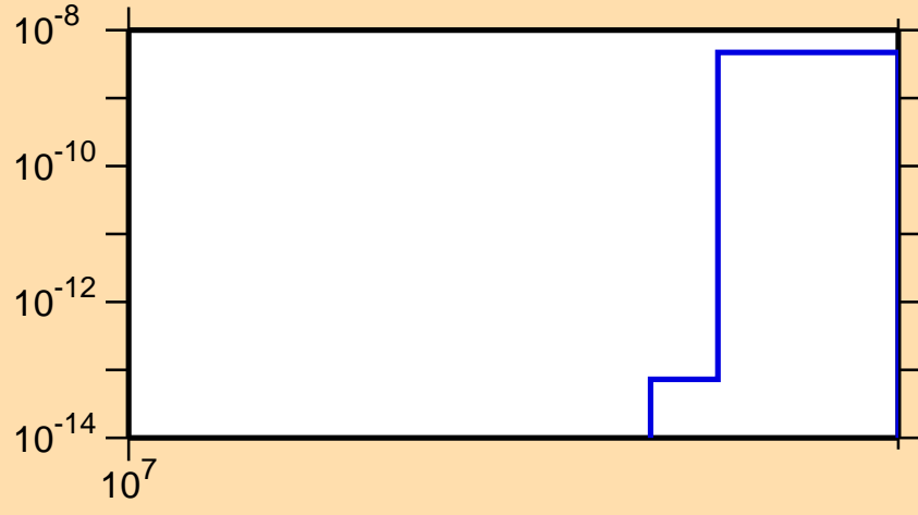
\sigma vs. E for ^{157}\text{Pm}(n,2np)
