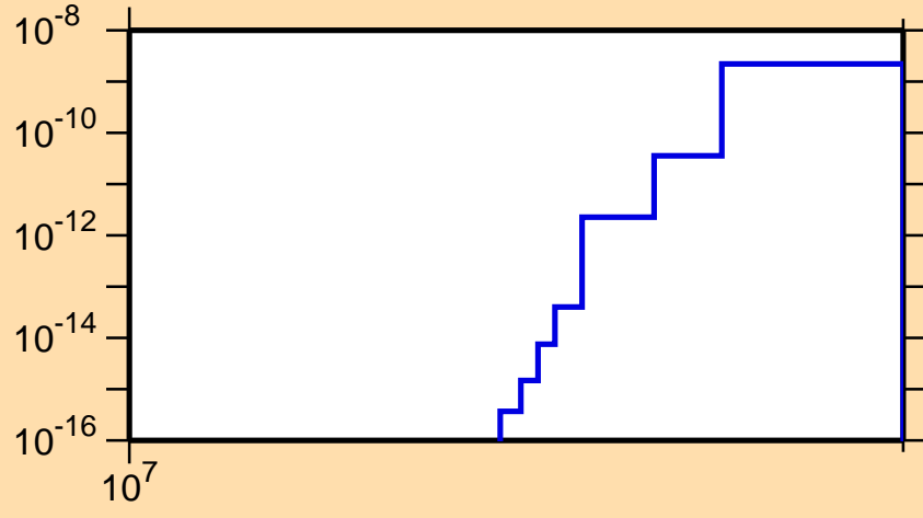
\sigma vs. E for ^{157}\text{Pm}(n,2n\alpha)
