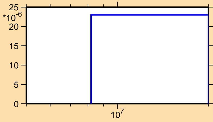
\sigma vs. E for ^{157}\text{Pm}(n,np)
