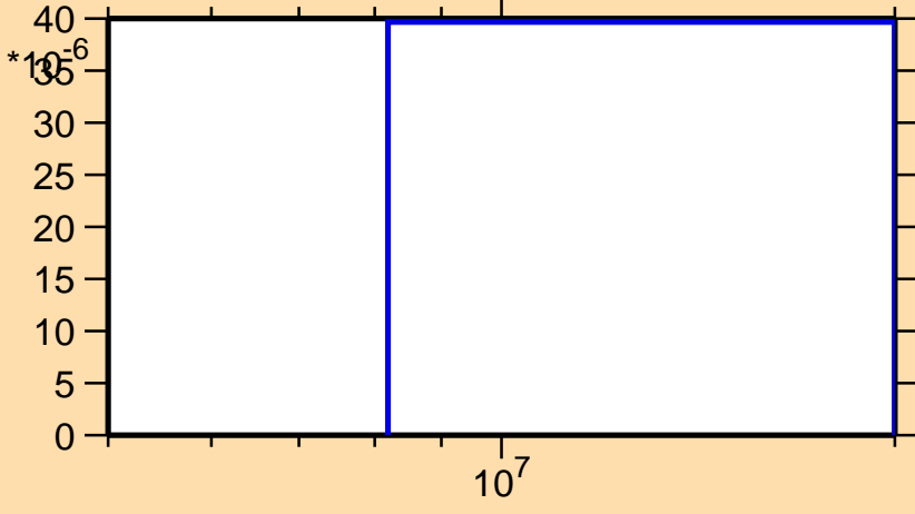
\sigma vs. E for ^{157}\text{Pm}(n,d)
