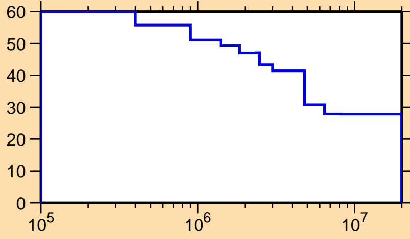
\Delta\sigma/\sigma vs. E for ^{157}\text{Pm}(n,n\text{onel.})
