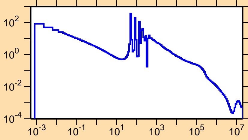
\sigma vs. E for ^{158}\text{Pm}(n,\gamma)
