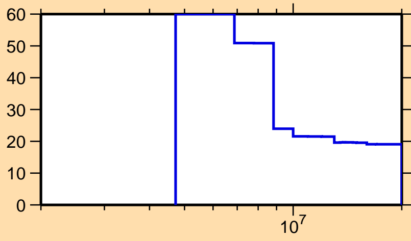
\Delta\sigma/\sigma vs. E for ^{158}\text{Pm}(n,\text{el.})
