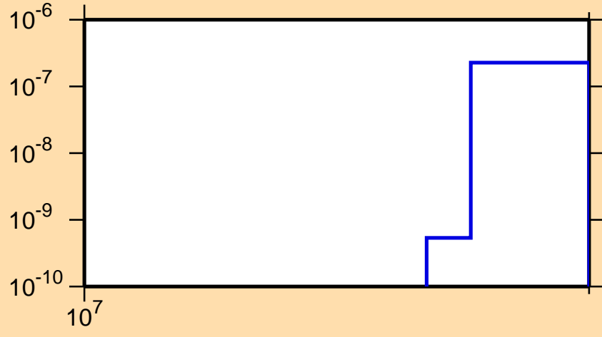
\sigma vs. E for ^{158}\text{Pm}(n,2np)
