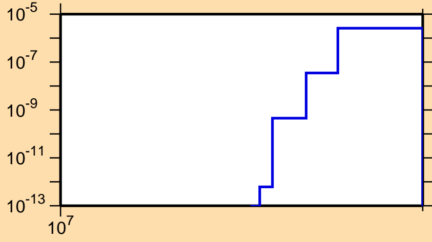
\sigma vs. E for ^{158}\text{Pm}(n,nt)
