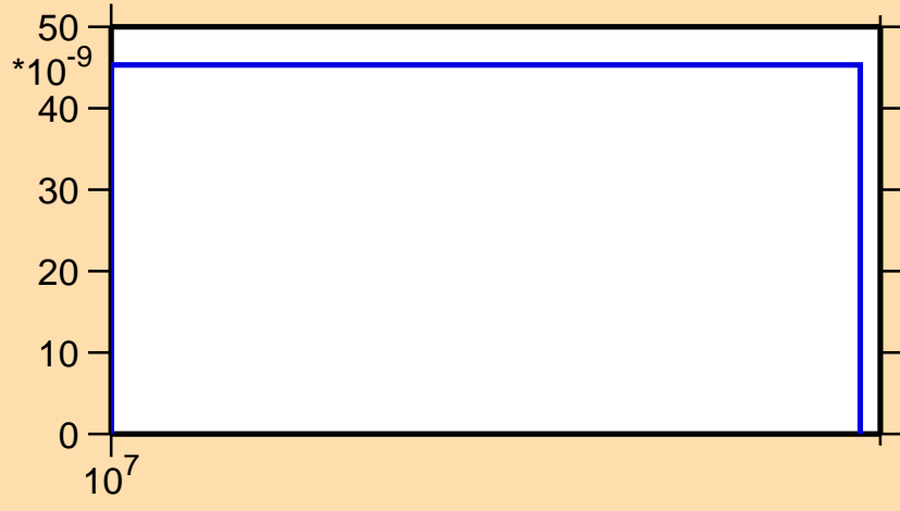
\sigma vs. E for ^{158}\text{Pm}(n,nd)
