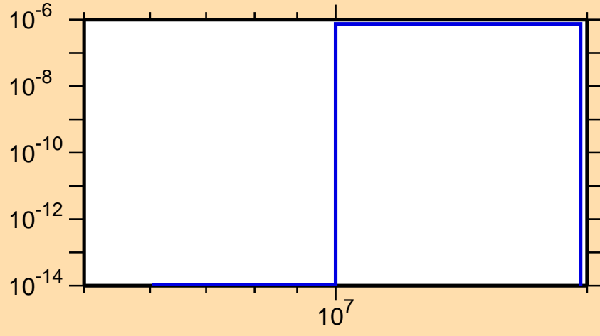
\sigma vs. E for ^{158}\text{Pm}(n,n\alpha)
