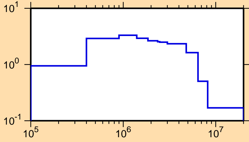
\sigma vs. E for ^{158}\text{Pm}(n,\text{inel.})
