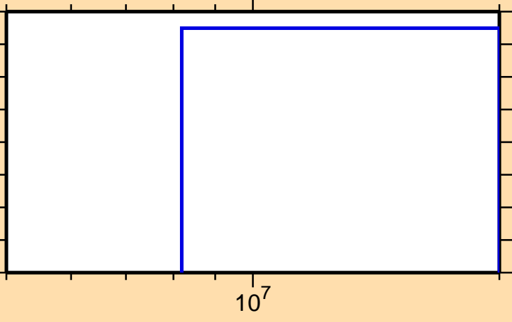
\sigma vs. E for ^{158}\text{Pm}(n,t)
