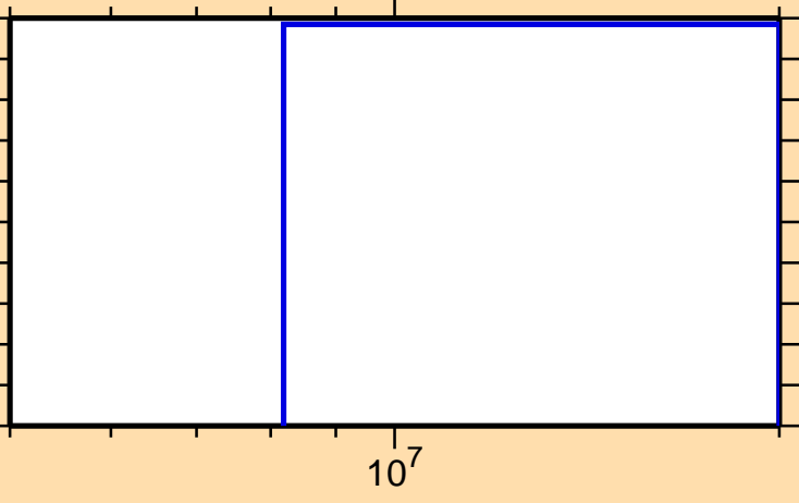
\sigma vs. E for ^{158}\text{Pm}(n,d)
