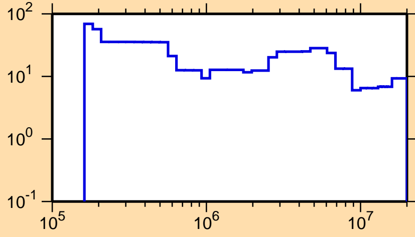
\Delta\sigma/\sigma vs. E for ^{159}\text{Pm}(n,\text{el.})
