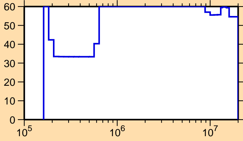
\Delta\sigma/\sigma vs. E for ^{159}\text{Pm}(n,n_1)
