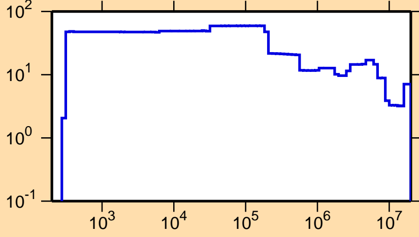
\Delta\sigma/\sigma vs. E for ^{159}\text{Pm}(n,\text{tot.})
