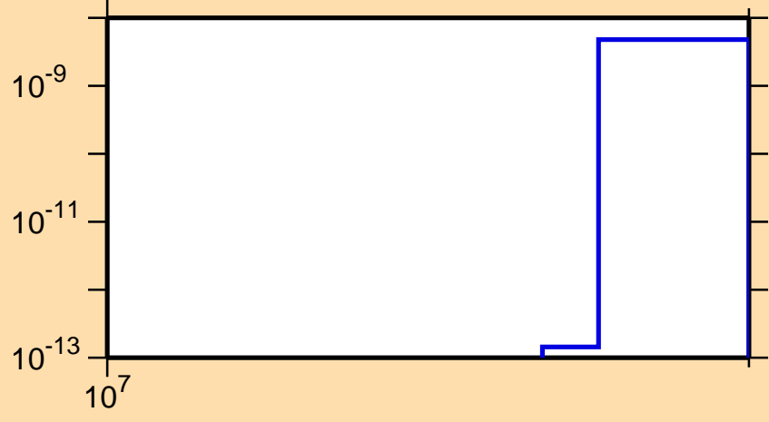
\sigma vs. E for ^{159}\text{Pm}(n,2np)
