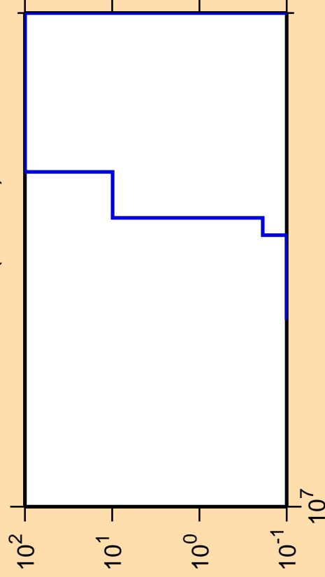
\Delta\sigma/\sigma vs. E for ^{159}\text{Pm}(n,2n\alpha)
