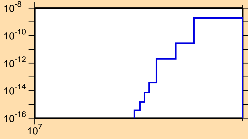
\sigma vs. E for ^{159}\text{Pm}(n,2n\alpha)
