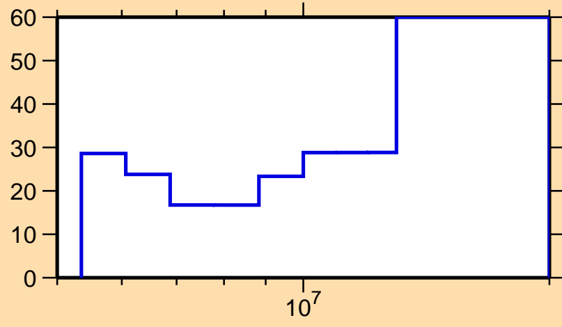
\Delta\sigma/\sigma vs. E for ^{159}\text{Pm}(n,2n)
