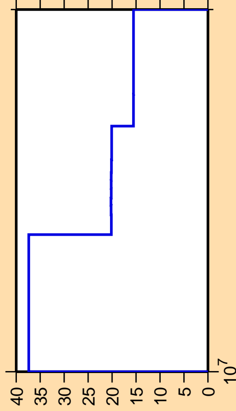
\Delta\sigma/\sigma vs. E for ^{159}\text{Pm}(n,3n)
