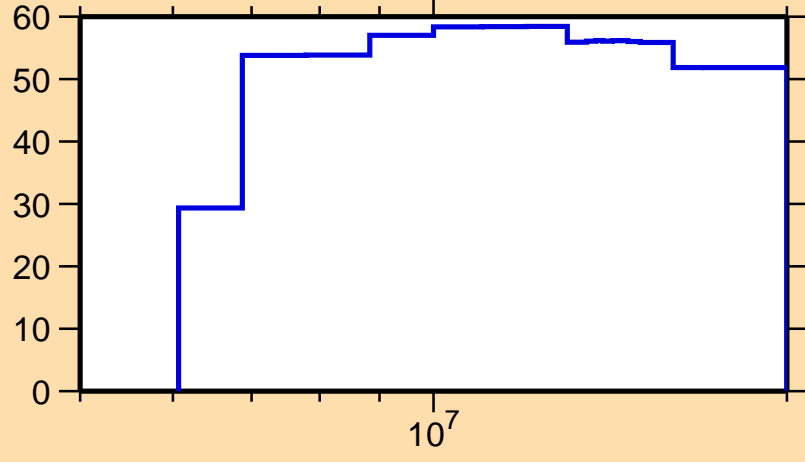
\Delta\sigma/\sigma vs. E for ^{159}\text{Pm}(n,\text{inel.})
