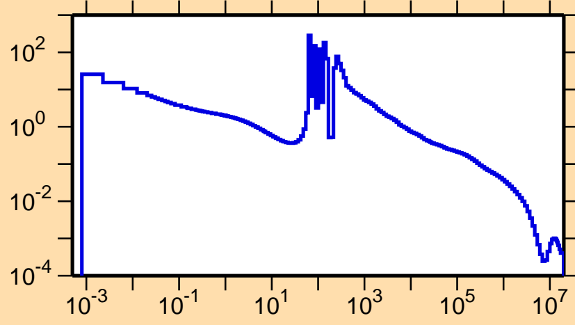
\sigma vs. E for ^{159}\text{Pm}(n,\gamma)
