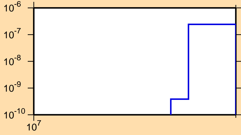
\sigma vs. E for ^{159}\text{Pm}(n,\text{nd})
