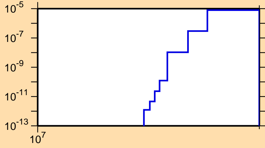
\sigma vs. E for ^{159}\text{Pm}(n,nt)
