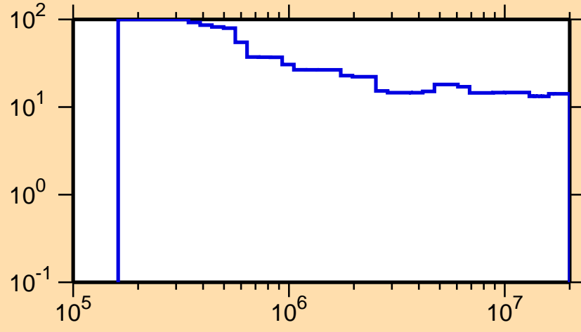
\Delta\sigma/\sigma vs. E for ^{159}\text{Pm}(n,\text{nonel.})
