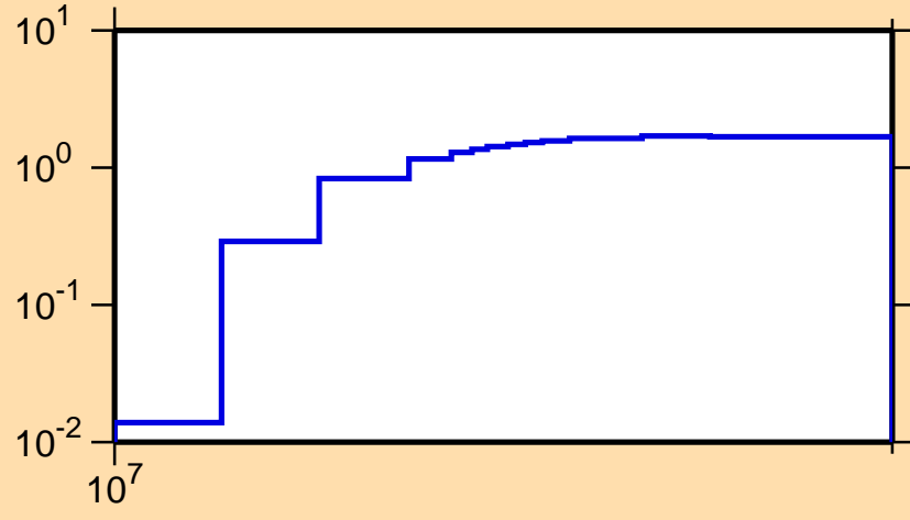
\sigma vs. E for ^{159}\text{Pm}(n,3n)
