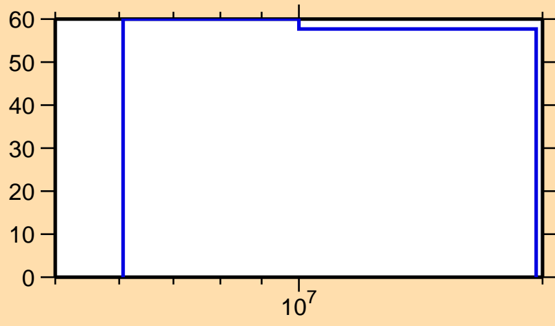
\Delta\sigma/\sigma vs. E for ^{159}\text{Pm}(n,n_1)
