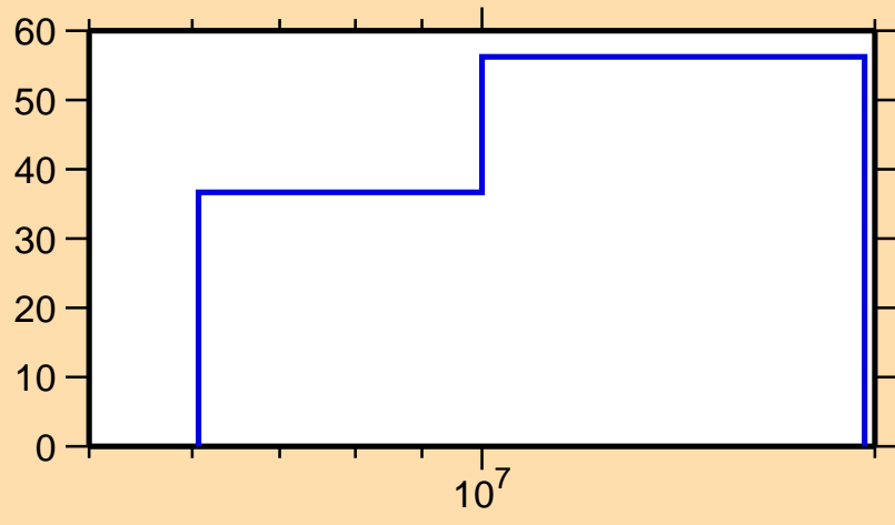
\Delta\sigma/\sigma vs. E for ^{159}\text{Pm}(n,\text{inel.})
