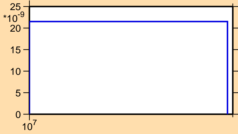
\sigma vs. E for ^{160}\text{Pm}(n,nd)
