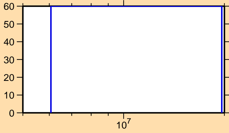
\Delta\sigma/\sigma vs. E for ^{160}\text{Pm}(n,n\text{cont.})
