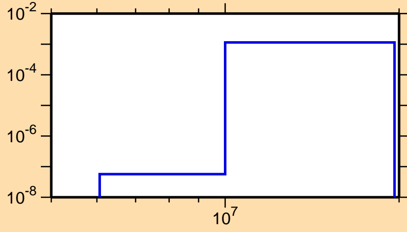
\sigma vs. E for ^{160}\text{Pm}(n,p)
