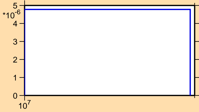
\sigma vs. E for ^{160}\text{Pm}(n,np)
