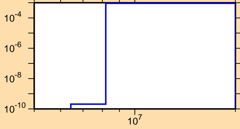
\sigma vs. E for ^{160}\text{Pm}(n,p)
