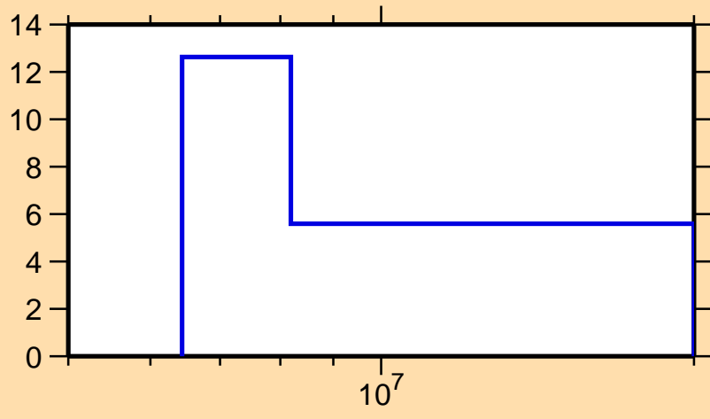
\Delta\sigma/\sigma vs. E for ^{160}\text{Pm}(n,el.)
