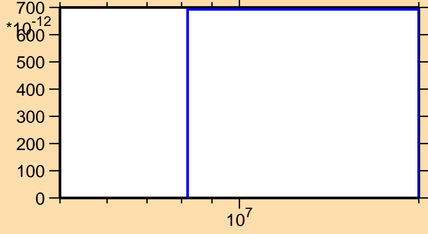
\sigma vs. E for ^{160}\text{Pm}(n,2np)
