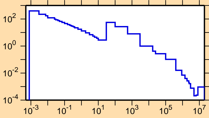
\sigma vs. E for ^{160}\text{Pm}(n,\gamma)
