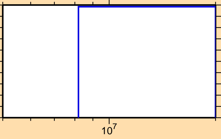
\sigma vs. E for ^{160}\text{Pm}(n,nd)
