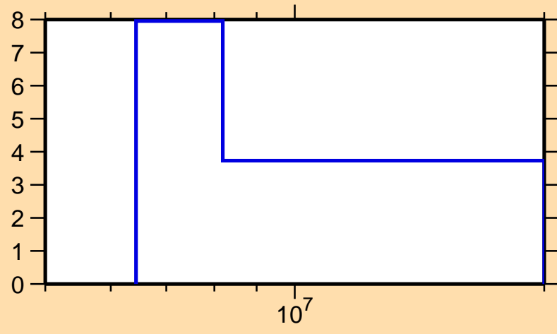
\Delta\sigma/\sigma vs. E for ^{160}\text{Pm}(n,\text{tot.})
