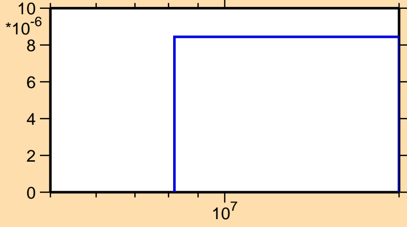
\sigma vs. E for ^{160}\text{Pm}(n,d)
