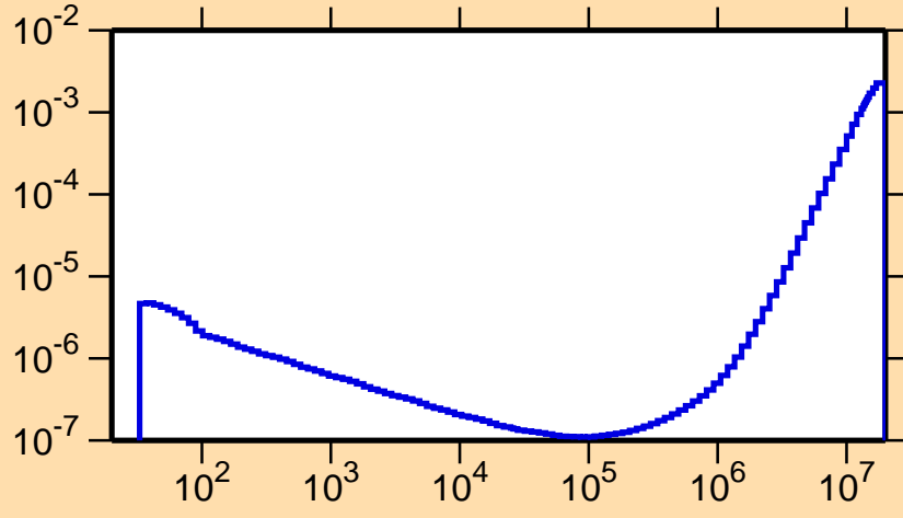
\sigma vs. E for ^{195}\text{Po}(n, p\alpha)
