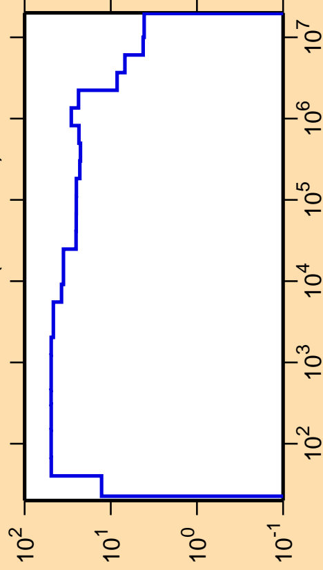
\Delta\sigma/\sigma vs. E for ^{195}\text{Po}(n,\text{nonel.})
