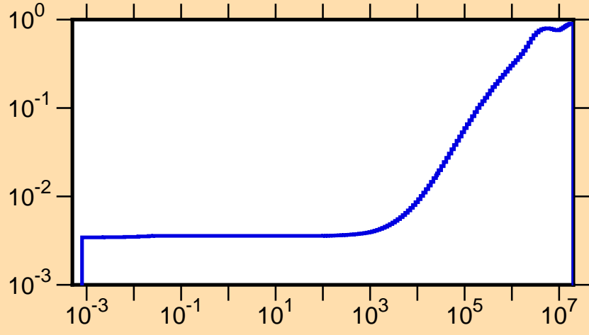
\mu vs. E for ^{196}\text{Po}(\text{mt251})
