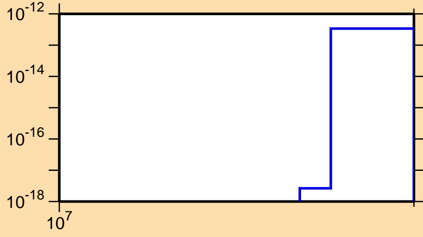
\sigma vs. E for ^{196}\text{Po}(n,3n\alpha)
