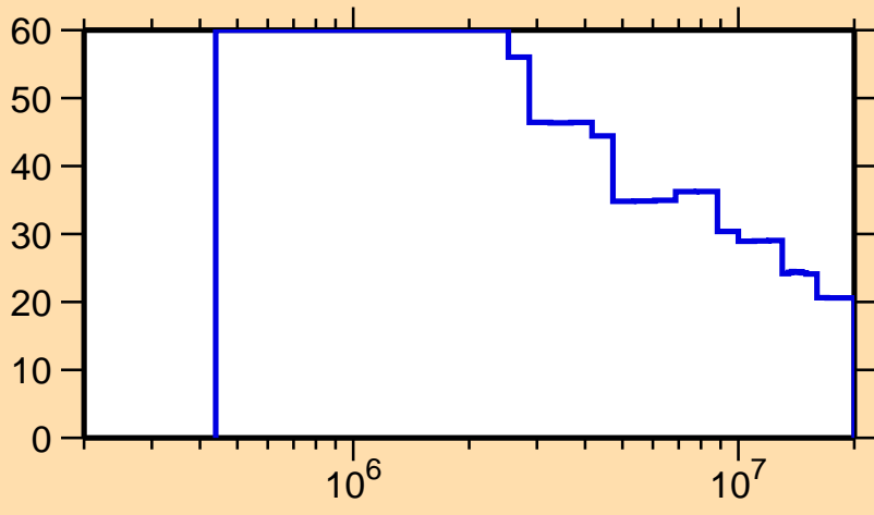
\Delta\sigma/\sigma vs. E for ^{196}\text{Po}(n,n_1)
