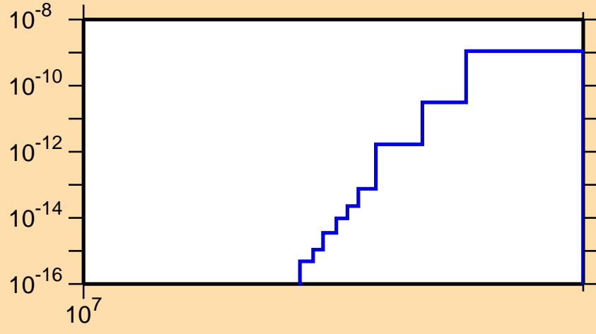
\sigma vs. E for ^{196}\text{Po}(n,\text{pt})
