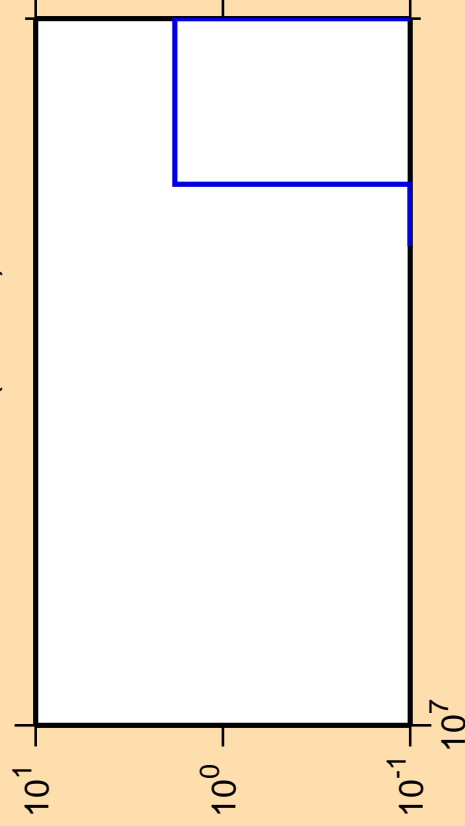
\Delta\sigma/\sigma vs. E for ^{196}\text{Po}(n,3n\alpha)
