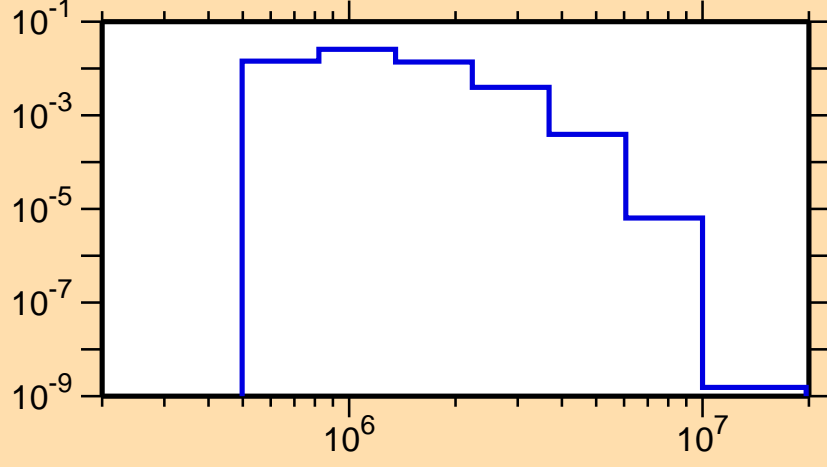
\sigma vs. E for ^{196}\text{Po}(n,n_2)
