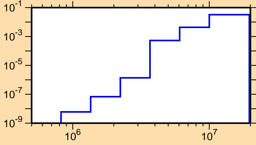
\sigma vs. E for ^{196}\text{Po}(n,n\alpha)
