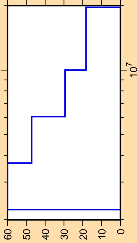
\Delta\sigma/\sigma vs. E for ^{196}\text{Po}(n,n\text{cont.})
