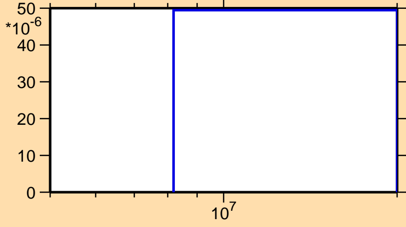
\sigma vs. E for ^{196}\text{Po}(n,t)
