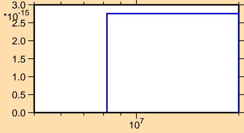
\sigma vs. E for ^{196}\text{Po}(n,3n\alpha)
