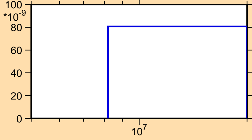
\sigma vs. E for ^{196}\text{Po}(n,2np)
