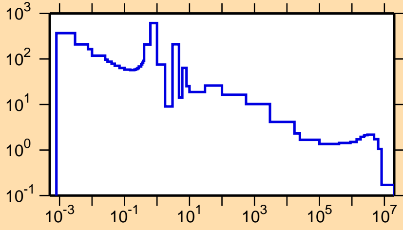
\sigma vs. E for ^{196}\text{Po}(n,\gamma)
