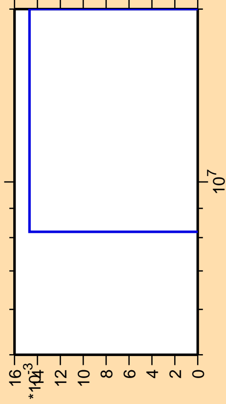
\Delta\sigma/\sigma vs. E for ^{196}\text{Po}(n,3n\alpha)
