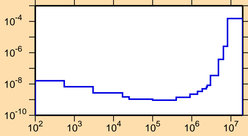
\sigma vs. E for ^{196}\text{Po}(n,p\alpha)
