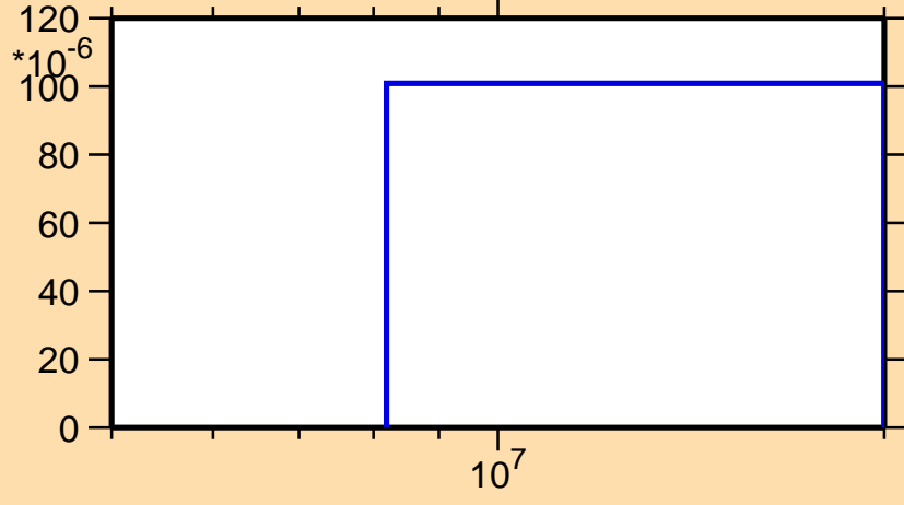
\sigma vs. E for ^{196}\text{Po}(n,2n\alpha)
