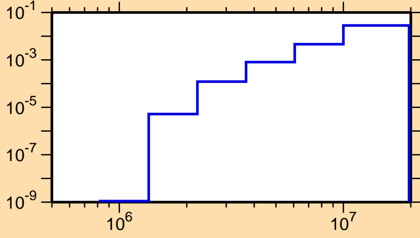
\sigma vs. E for ^{197}\text{Po}(n,n\alpha)
