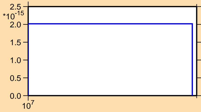
\sigma vs. E for ^{197}\text{Po}(n,3n\alpha)
