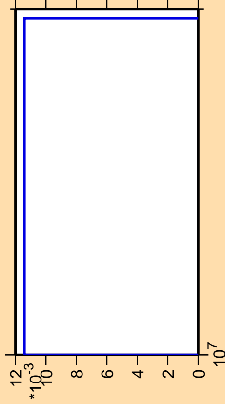
\Delta\sigma/\sigma vs. E for ^{197}\text{Po}(n,3n\alpha)
