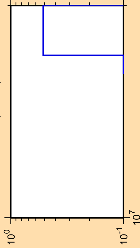
\Delta\sigma/\sigma vs. E for ^{197}\text{Po}(n,3n\alpha)
