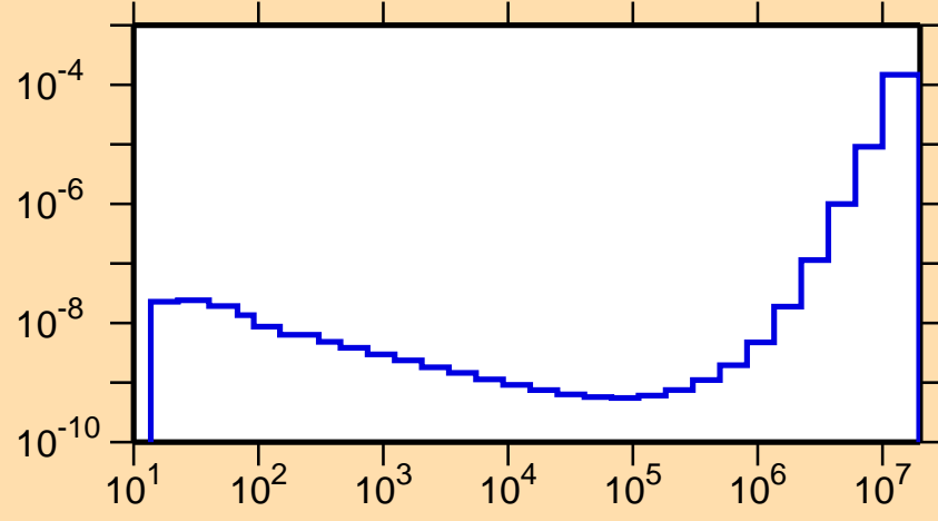
\sigma vs. E for ^{197}\text{Po}(n,p\alpha)
