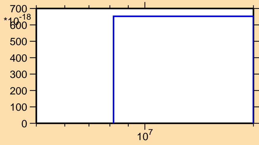
\sigma vs. E for ^{197}\text{Po}(n,3n\alpha)
