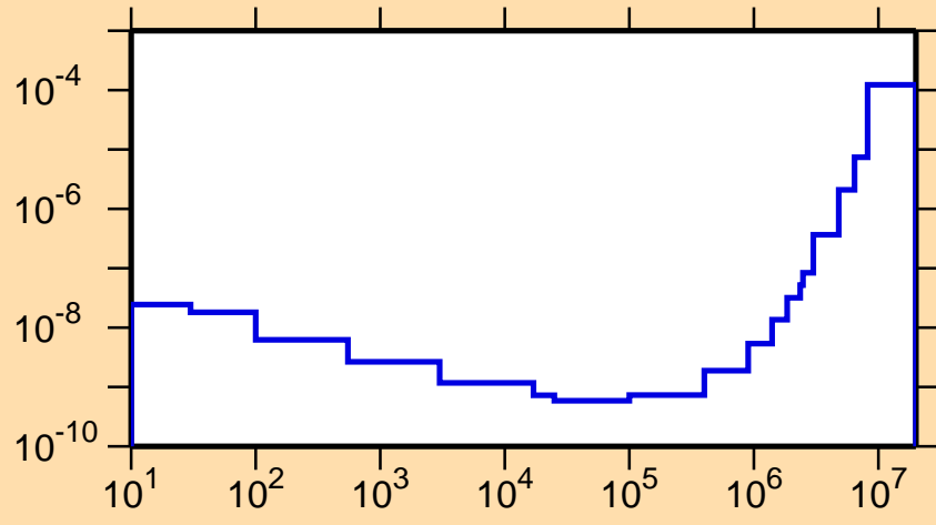
\sigma vs. E for ^{197}\text{Po}(n,p\alpha)
