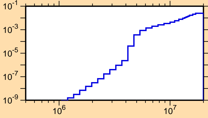
\sigma vs. E for ^{198}\text{Po}(n,n\alpha)
