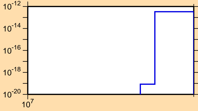
\sigma vs. E for ^{198}\text{Po}(n,3n\alpha)
