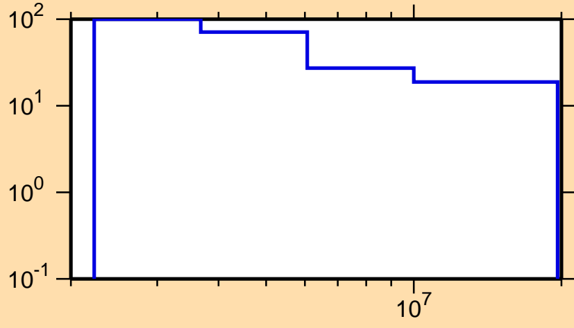
\Delta\sigma/\sigma vs. E for ^{198}\text{Po}(n,n\text{cont.})
