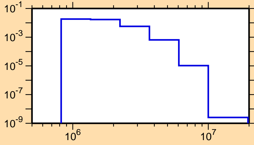
\sigma vs. E for ^{198}\text{Po}(n,n_2)
