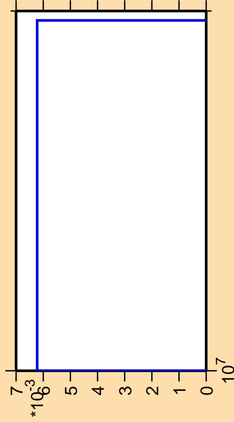
\Delta\sigma/\sigma vs. E for ^{198}\text{Po}(n,3n\alpha)
