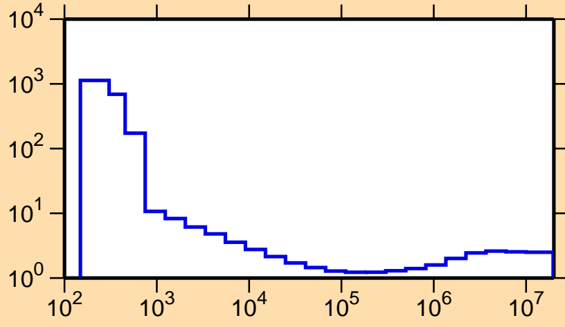
\sigma vs. E for ^{198}\text{Po}(n,\text{nonel.})
