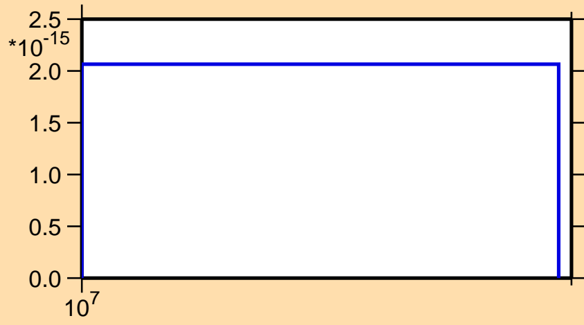
\sigma vs. E for ^{198}\text{Po}(n,3n\alpha)
