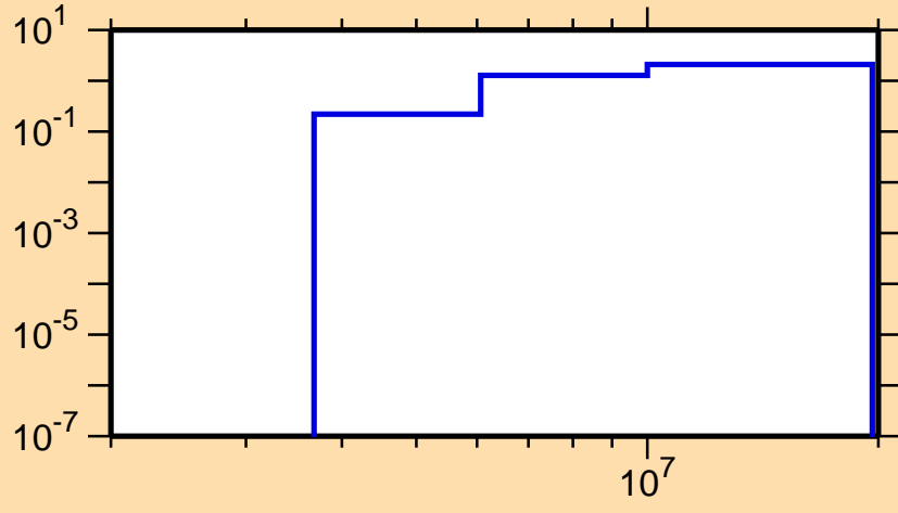
\sigma vs. E for ^{198}\text{Po}(n,n\text{cont.})
