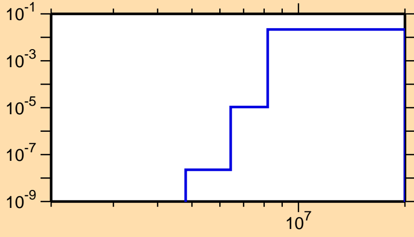
\sigma vs. E for ^{198}\text{Po}(n,np)
