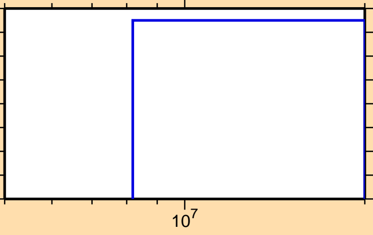
\sigma vs. E for ^{198}\text{Po}(n,\text{nd})
