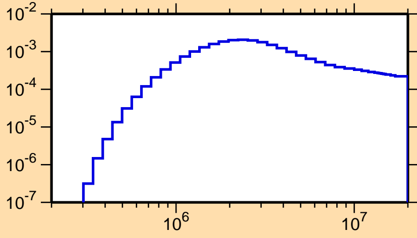
\sigma vs. E for ^{199}\text{Po}(n,n_2)
