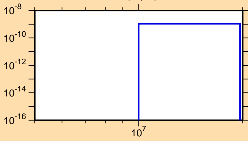
\sigma vs. E for ^{199}\text{Po}(n,pd)
