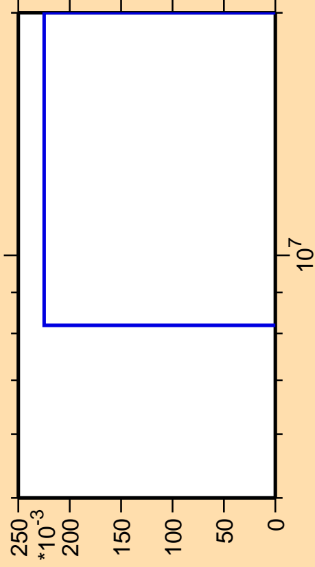
\Delta\sigma/\sigma vs. E for ^{199}\text{Po}(n,3n\alpha)
