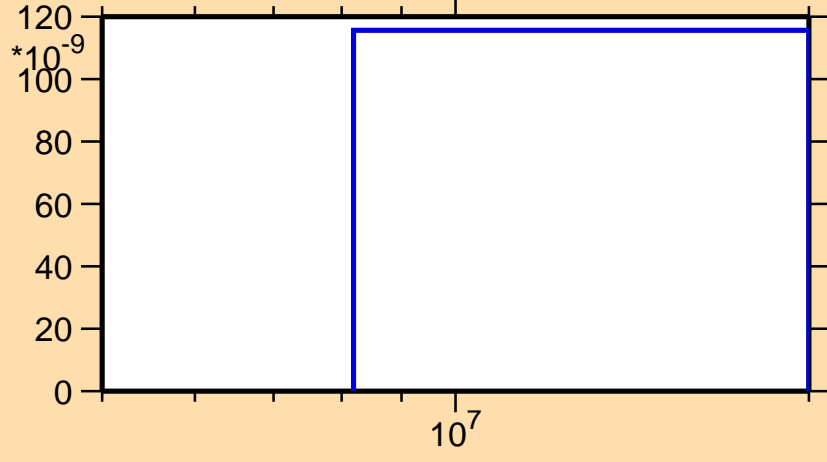
\sigma vs. E for ^{199}\text{Po}(n,3n)
