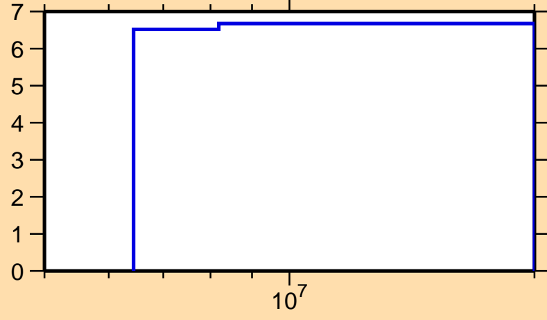
\Delta\sigma/\sigma vs. E for ^{199}\text{Po}(n,\text{nonel.})
