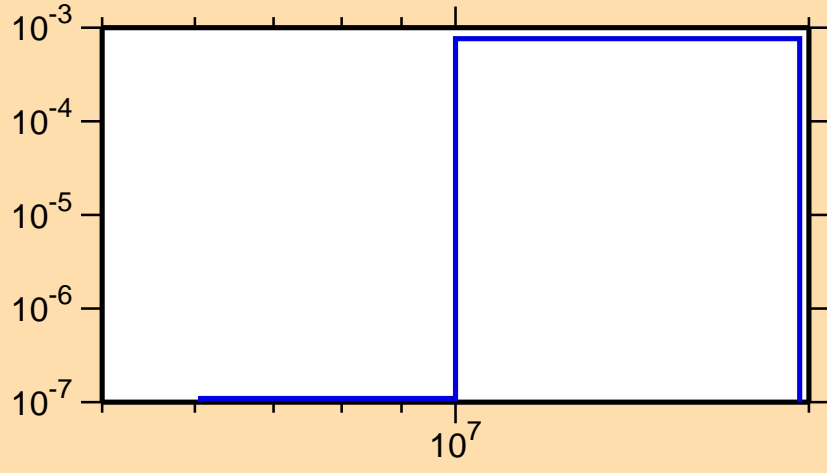
\sigma vs. E for ^{199}\text{Po}(n,2n\alpha)
