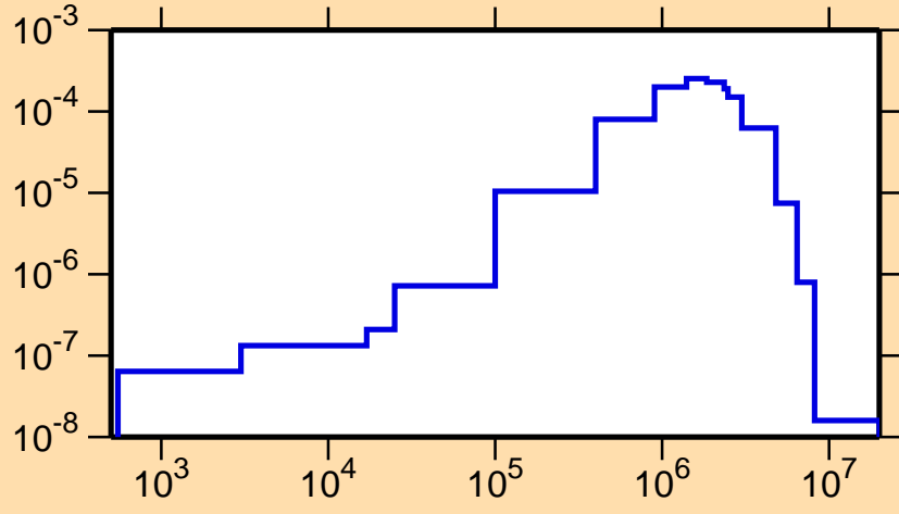
\sigma vs. E for ^{199}\text{Po}(n,n_1)
