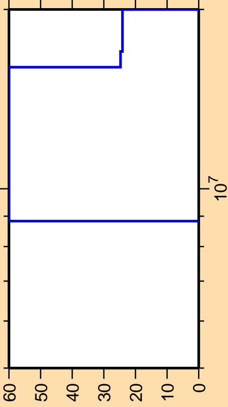
\Delta\sigma/\sigma vs. E for ^{200}\text{Po}(n,2n)
