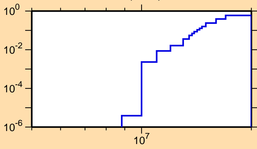
\sigma vs. E for ^{200}\text{Po}(n,2n)
