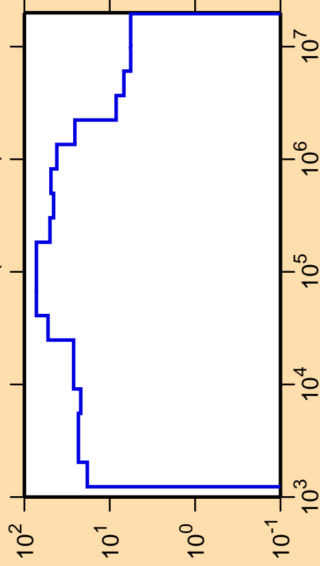
\Delta\sigma/\sigma vs. E for ^{200}\text{Po}(n,\text{nonel.})
