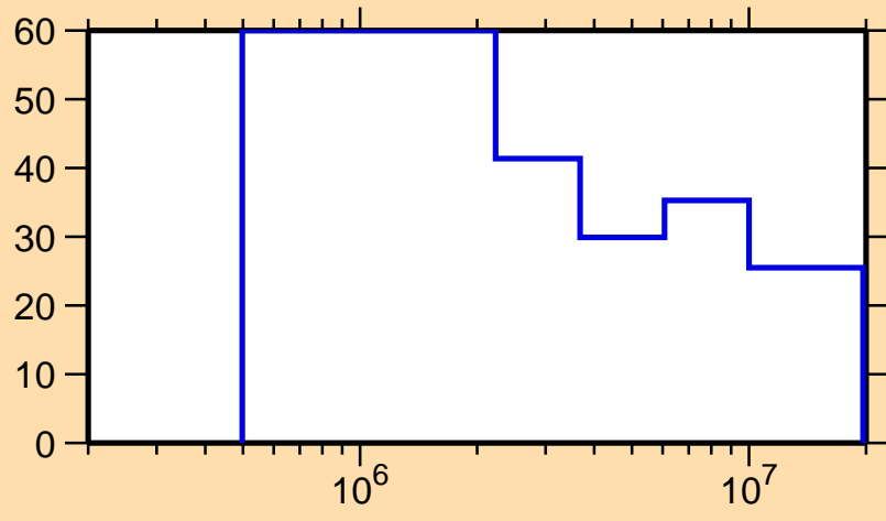
\Delta\sigma/\sigma vs. E for ^{200}\text{Po}(n,n_1)
