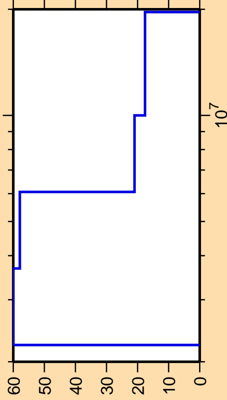
\Delta\sigma/\sigma vs. E for ^{200}\text{Po}(n,n\text{cont.})
