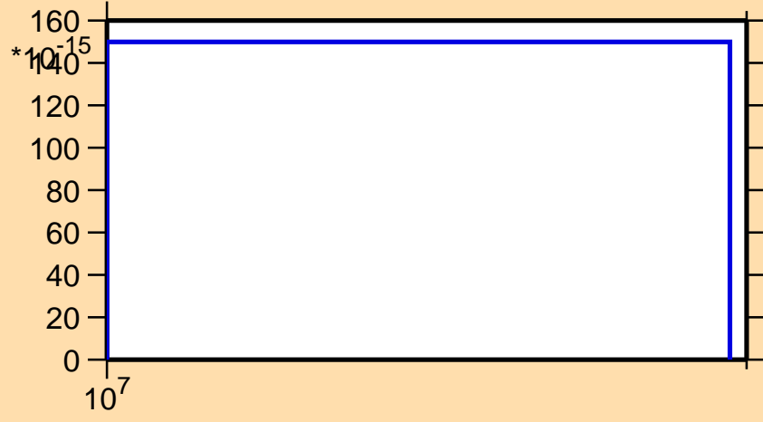
\sigma vs. E for ^{200}\text{Po}(n,\text{pt})
