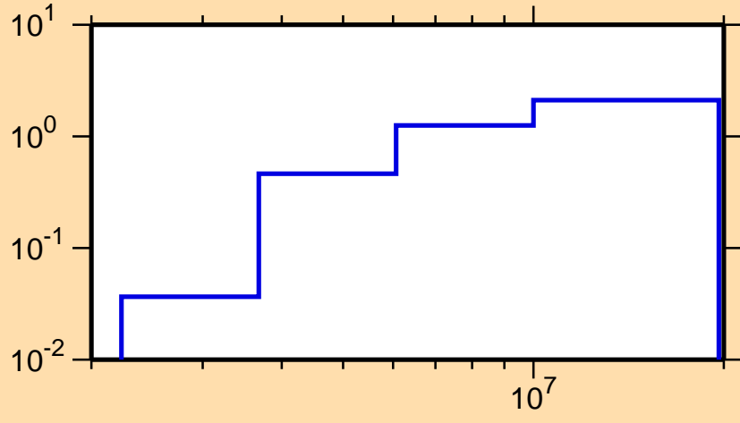
\sigma vs. E for ^{200}\text{Po}(n,n\text{cont.})
