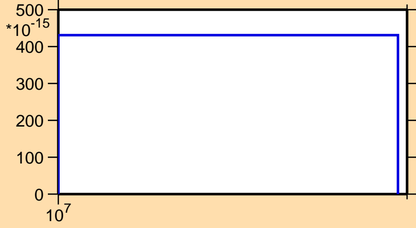
\sigma vs. E for ^{200}\text{Po}(n,3n\alpha)
