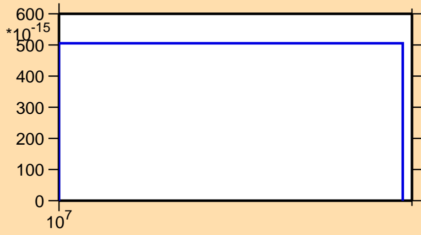
\sigma vs. E for ^{200}\text{Po}(n,nt)
