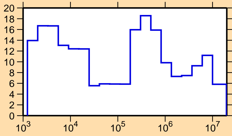
\Delta\sigma/\sigma vs. E for ^{200}\text{Po}(n,el.)
