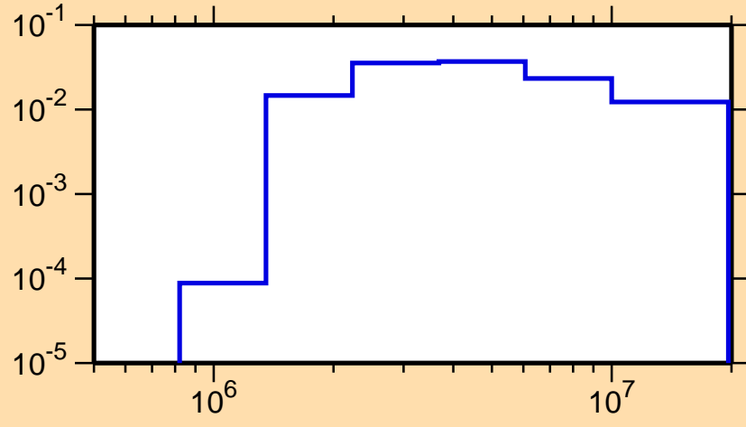
\sigma vs. E for ^{200}\text{Po}(n,n_3)
