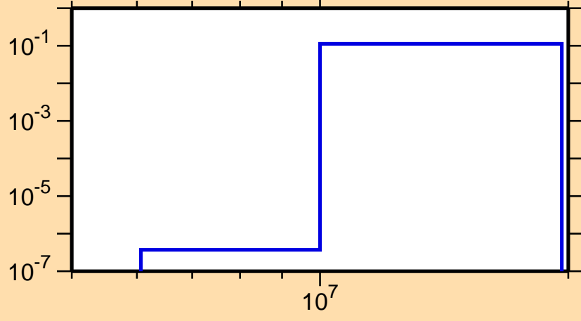
\sigma vs. E for ^{200}\text{Po}(n,2n)
