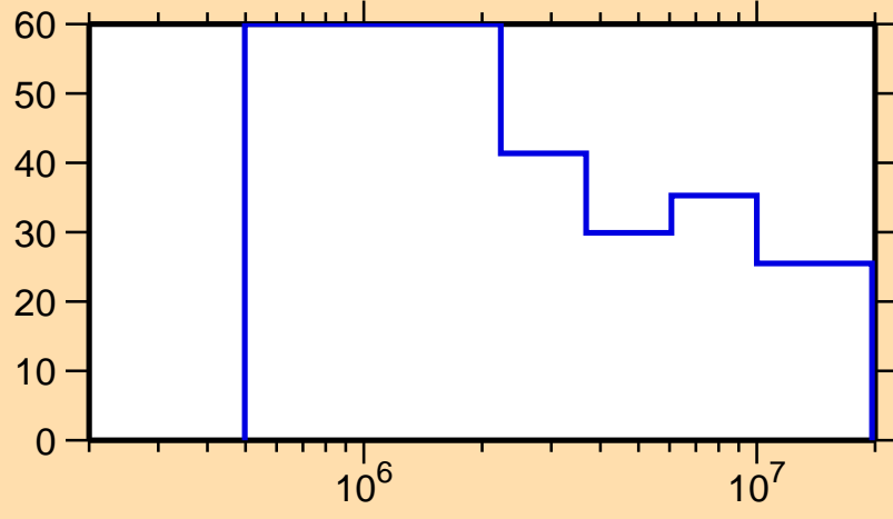
\Delta\sigma/\sigma vs. E for ^{200}\text{Po}(n,n_1)
