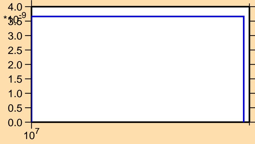
\sigma vs. E for ^{200}\text{Po}(n,2np)
