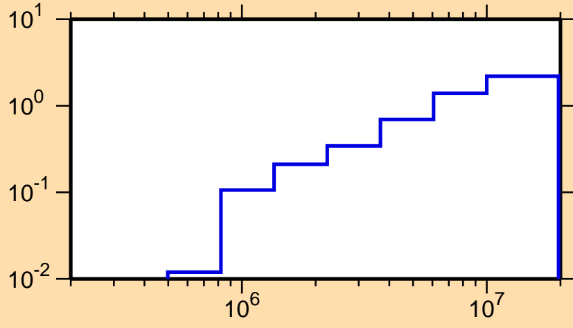
\sigma vs. E for ^{200}\text{Po}(n,\text{inel.})
