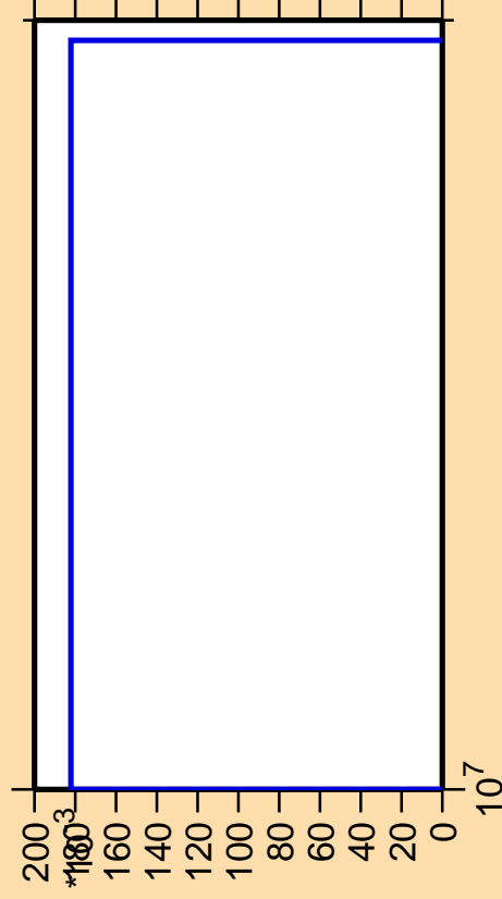
\Delta\sigma/\sigma vs. E for ^{200}\text{Po}(\text{mt } 34)
