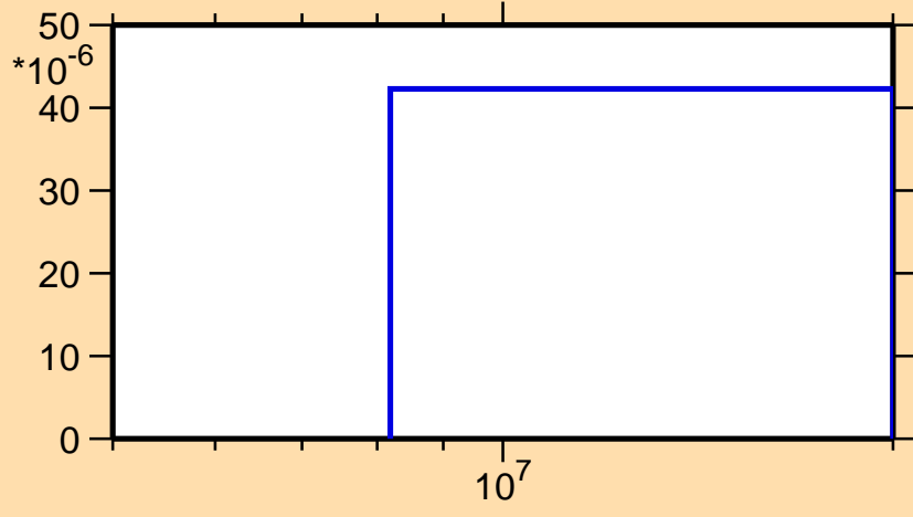
\sigma vs. E for ^{200}\text{Po}(n,t)
