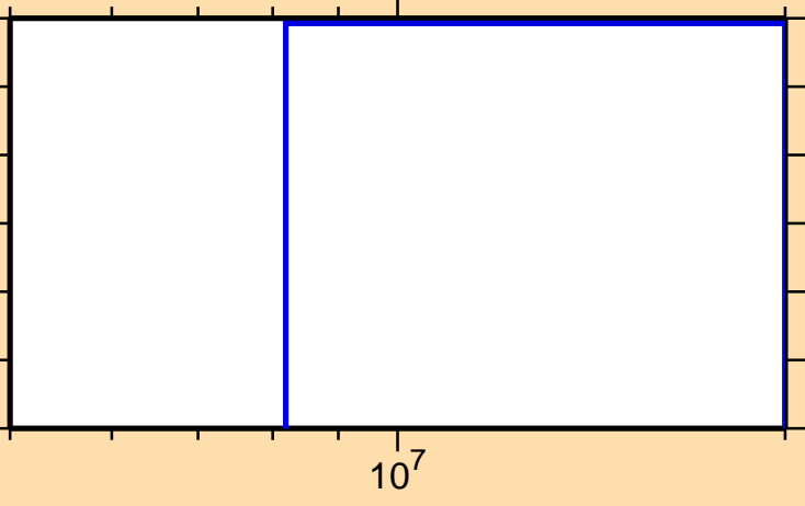
\sigma vs. E for ^{200}\text{Po}(n,nt)
