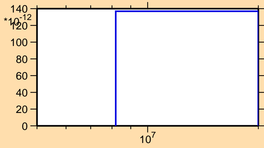
\sigma vs. E for ^{200}\text{Po}(n,\text{pd})
