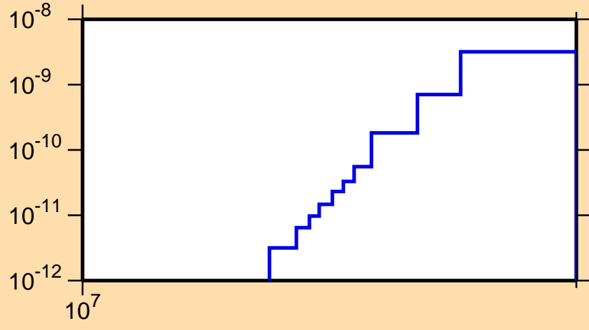
\sigma vs. E for ^{201}\text{Po}(\text{mt117})
