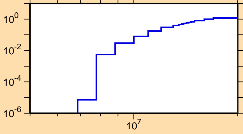
\sigma vs. E for ^{201}\text{Po}(n,2n)
