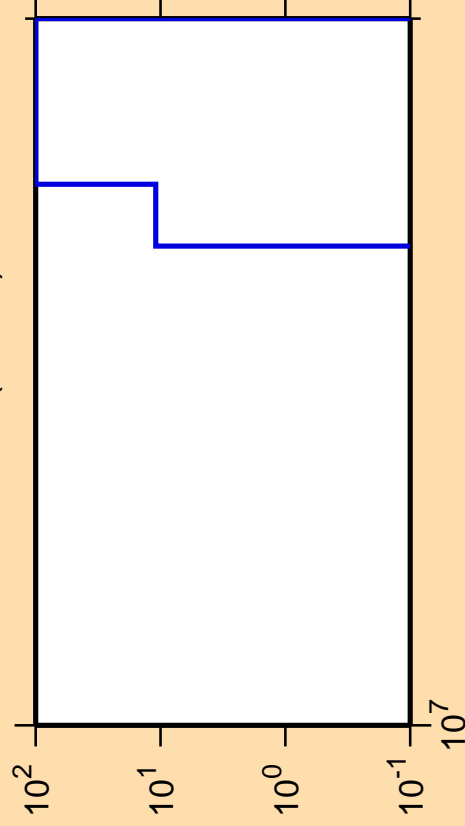
\Delta\sigma/\sigma vs. E for ^{201}\text{Po} (mt 34)
