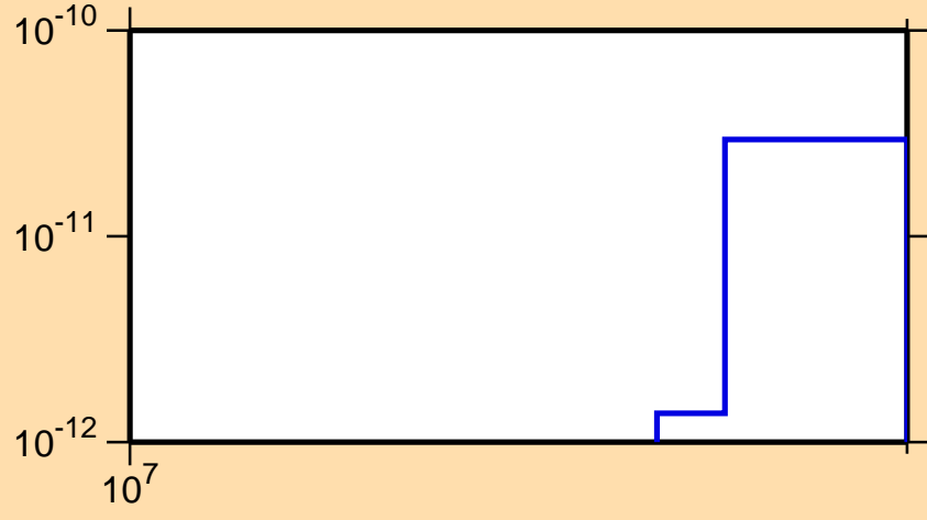
\sigma vs. E for ^{201}\text{Po} (mt 34)
