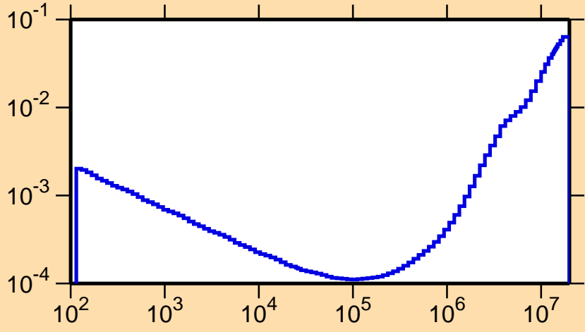
\sigma vs. E for ^{201}\text{Po}(n,p)
