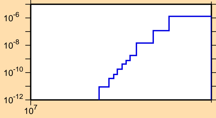
\sigma vs. E for ^{201}\text{Po}(n,\text{nd})
