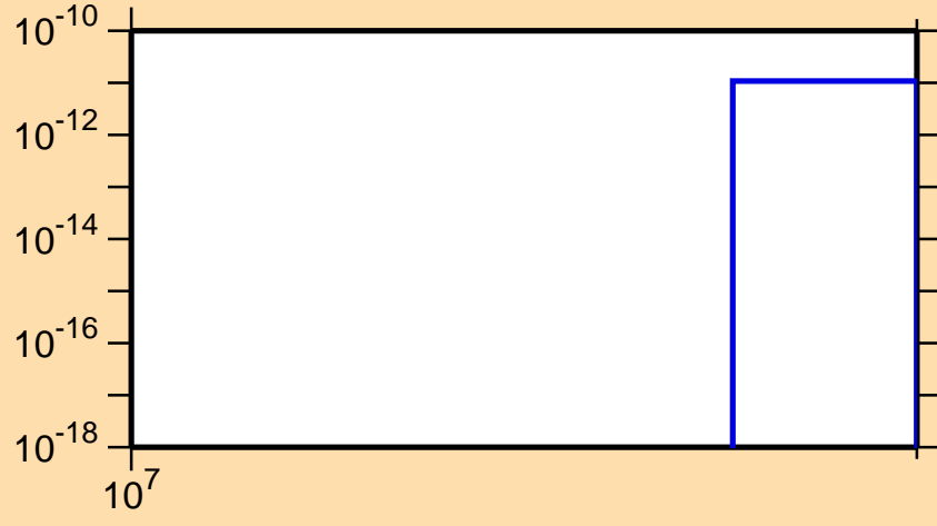
\sigma vs. E for ^{201}\text{Po}(n,3n\alpha)
