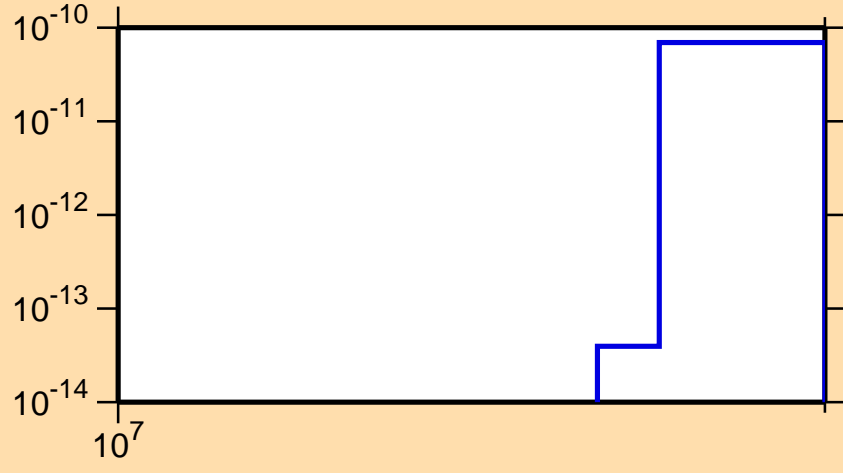
\sigma vs. E for ^{201}\text{Po}(n,nt)
