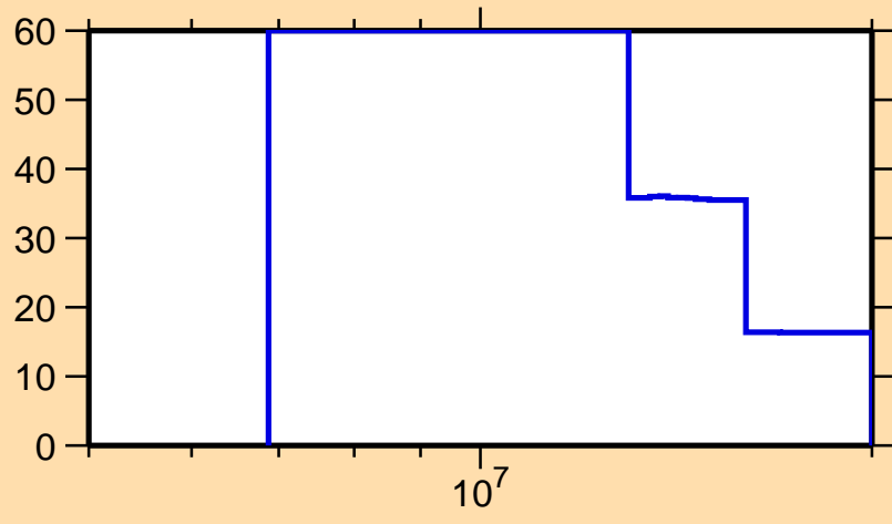
\Delta\sigma/\sigma vs. E for ^{201}\text{Po}(n,2n)
