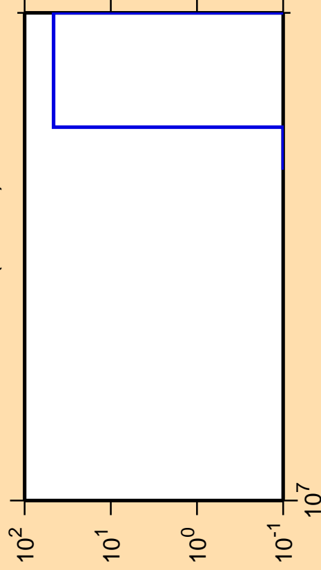
\Delta\sigma/\sigma vs. E for ^{201}\text{Po}(n,3n\alpha)
