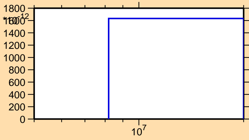
\sigma vs. E for ^{201}\text{Po}(\text{mt } 45)
