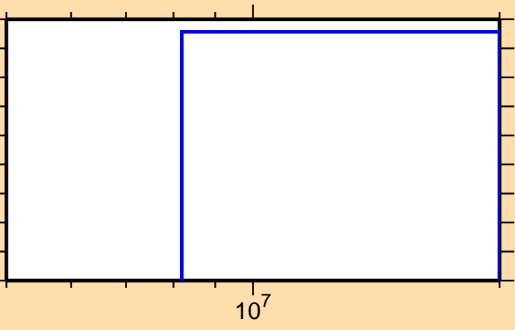
\sigma vs. E for ^{201}\text{Po}(n,\text{nd})
