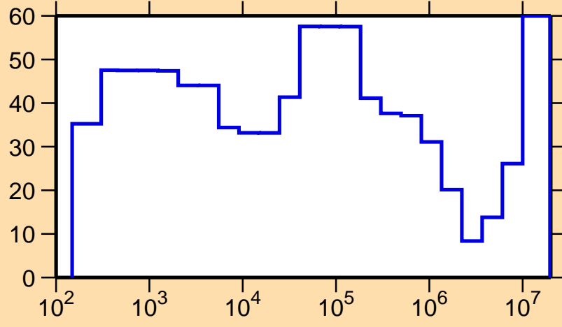
\Delta\sigma/\sigma vs. E for ^{201}\text{Po}(n,\gamma)
