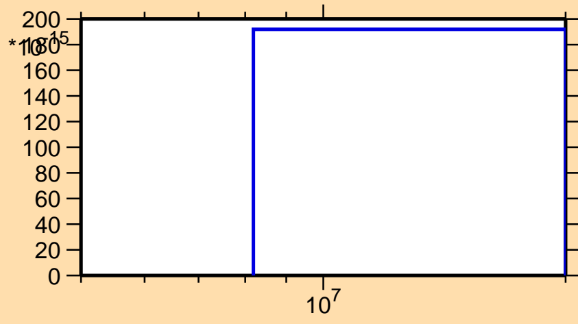
\sigma vs. E for ^{201}\text{Po}(\text{mt } 34)
