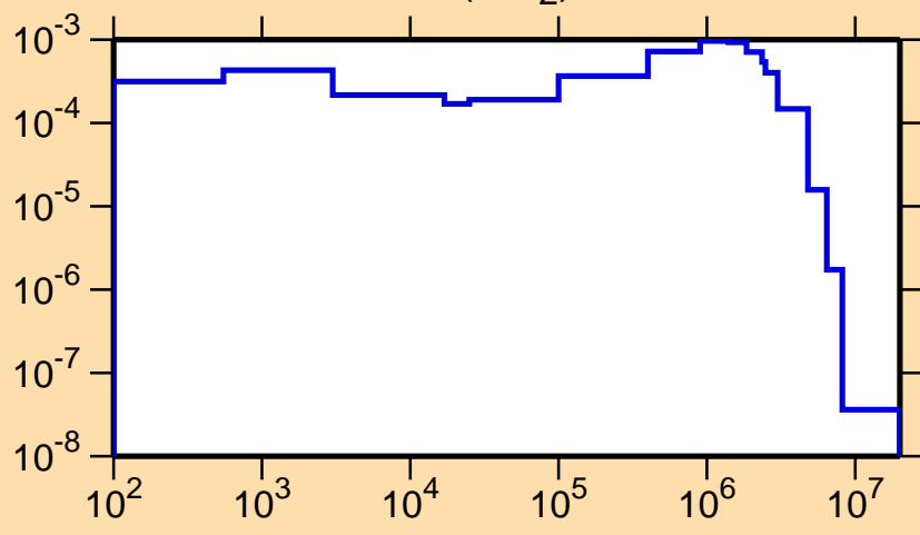
\sigma vs. E for ^{201}\text{Po}(n,n_2)
