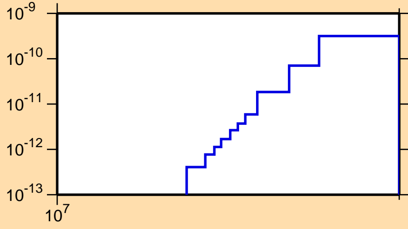
\sigma vs. E for ^{202}\text{Po}(\text{mt117})
