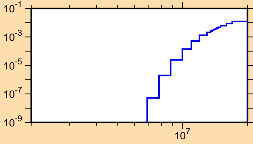
\sigma vs. E for ^{202}\text{Po}(n,np)
