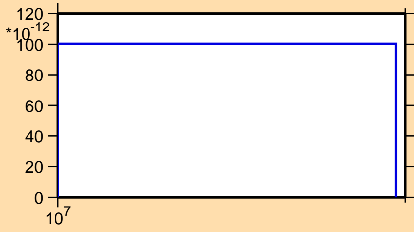
\sigma vs. E for ^{202}\text{Po} (mt 45)
