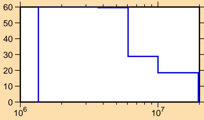
\Delta\sigma/\sigma vs. E for ^{202}\text{Po}(n,n\text{cont.})
