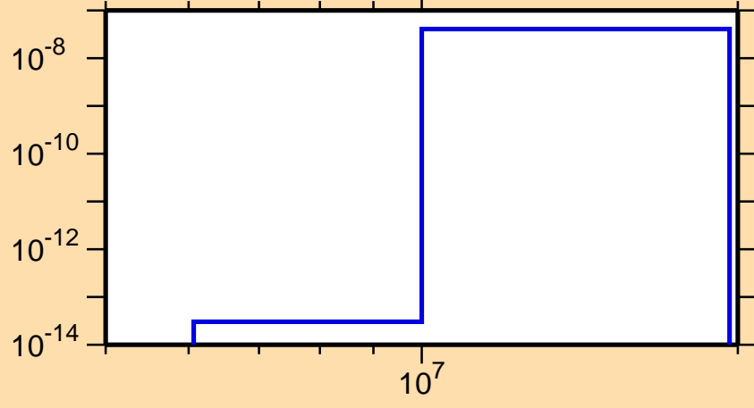
\sigma vs. E for ^{202}\text{Po}(n,\text{He}3)
