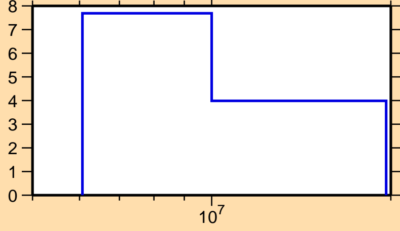
\Delta\sigma/\sigma vs. E for ^{202}\text{Po}(n,\text{tot.})
