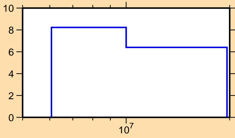
\Delta\sigma/\sigma vs. E for ^{202}\text{Po}(n,\text{nonel.})
