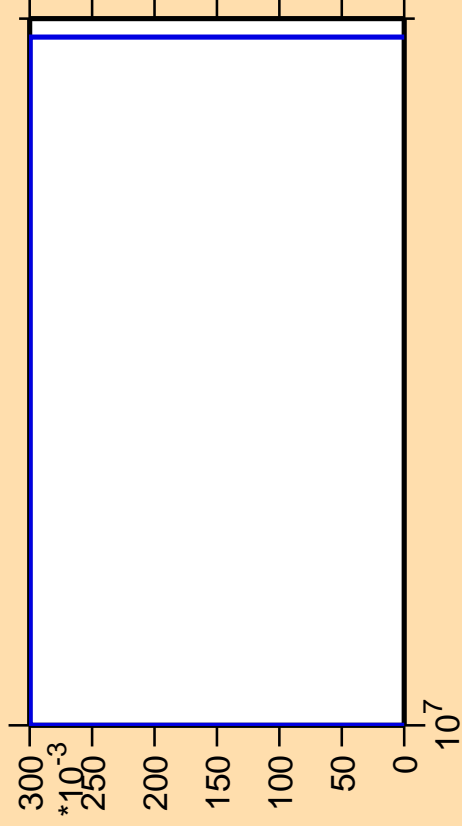
\Delta\sigma/\sigma vs. E for ^{202}\text{Po} (mt 34)
