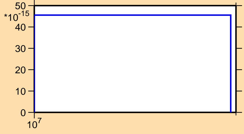
\sigma vs. E for ^{202}\text{Po} (mt 34)
