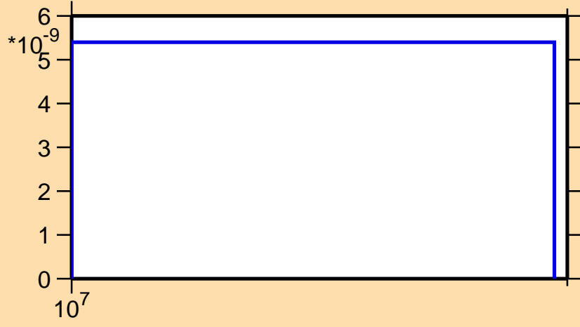
\sigma vs. E for ^{202}\text{Po}(n,2np)
