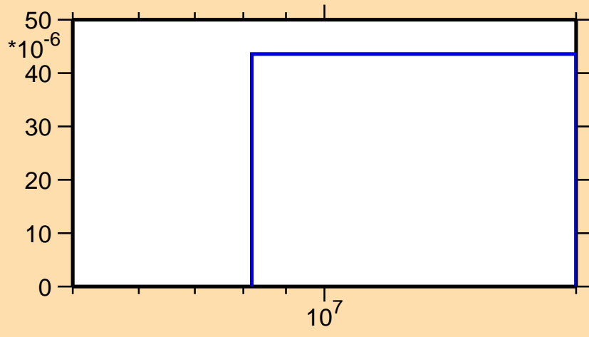
\sigma vs. E for ^{202}\text{Po}(n,t)
