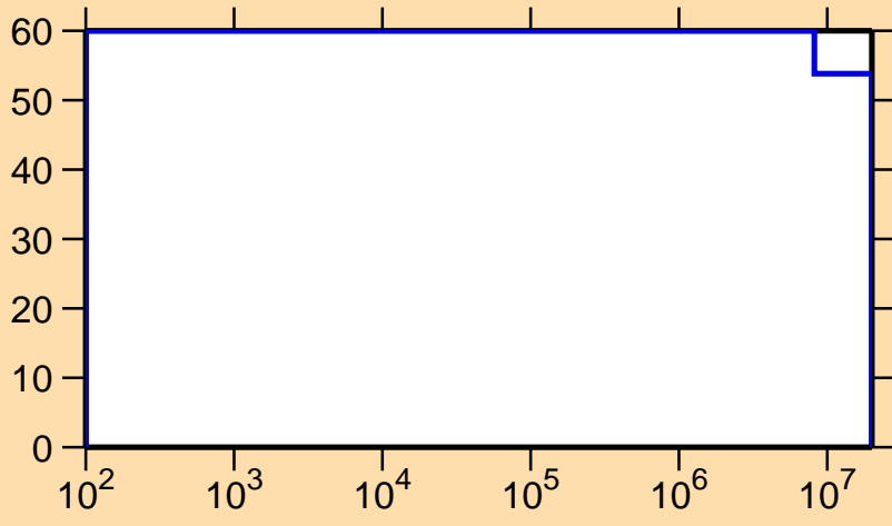
\Delta\sigma/\sigma vs. E for ^{202}\text{Po}(n,p)
