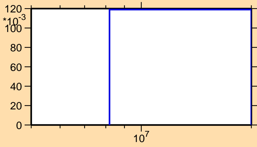
\sigma vs. E for ^{202}\text{Po}(n,2n)
