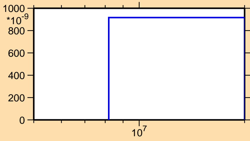
\sigma vs. E for ^{202}\text{Po}(n,3n)
