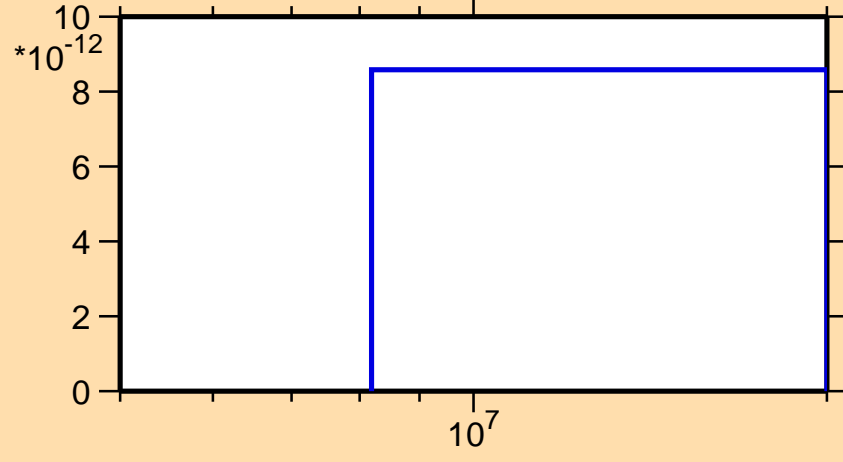
\sigma vs. E for ^{202}\text{Po}(\text{mt117})
