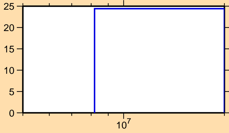
\Delta\sigma/\sigma vs. E for ^{202}\text{Po}(n,\text{inel.})
