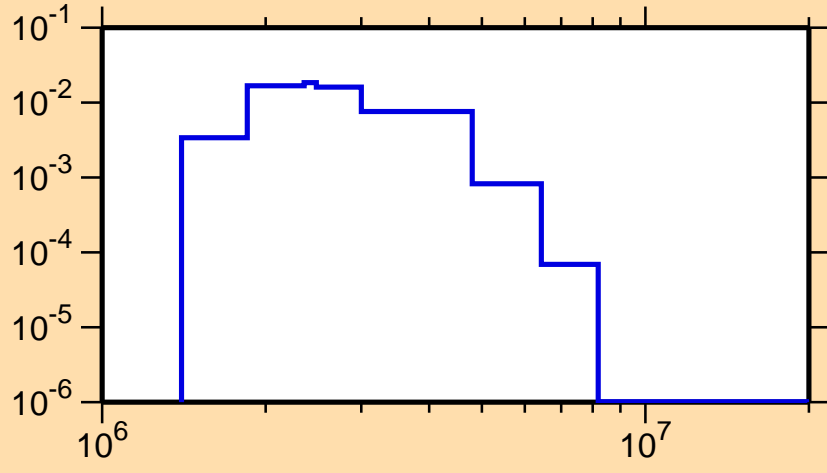
\sigma vs. E for ^{202}\text{Po}(n,n_4)
