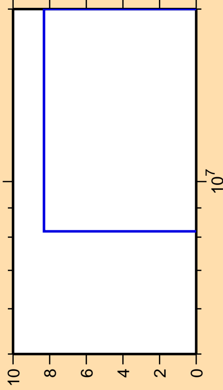
\Delta\sigma/\sigma vs. E for ^{202}\text{Po}(n,nt)
