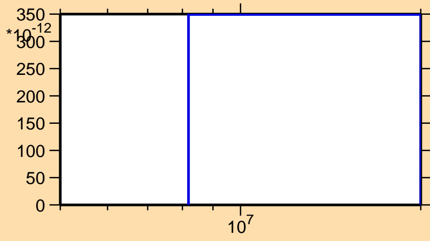
\sigma vs. E for ^{202}\text{Po}(n,3n\alpha)
