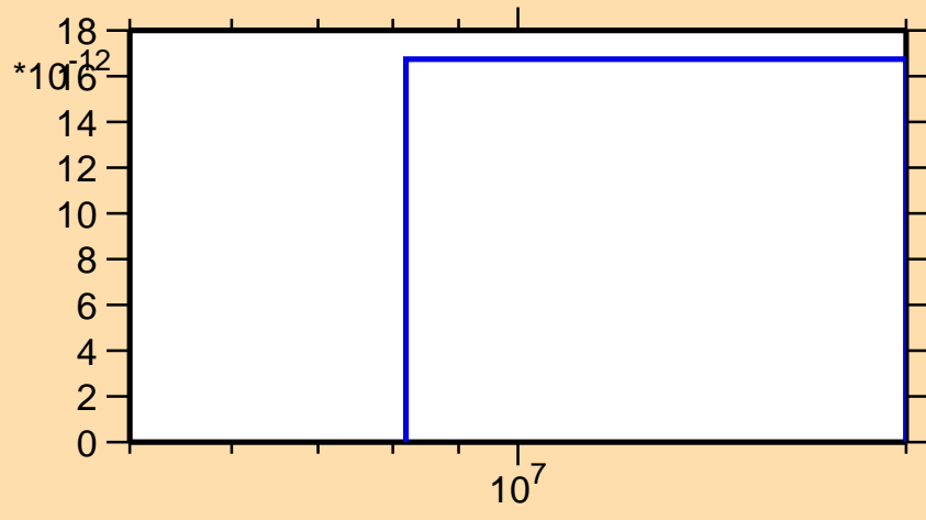
\sigma vs. E for ^{202}\text{Po}(n,\text{pd})
