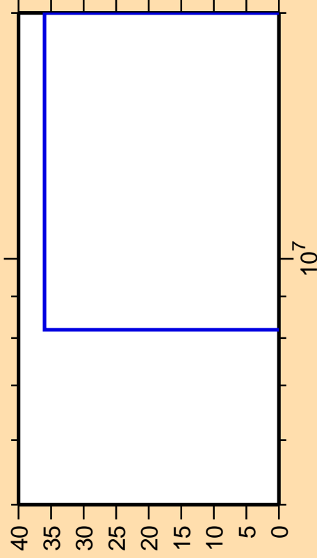
\Delta\sigma/\sigma vs. E for ^{202}\text{Po}(\text{mt117})
