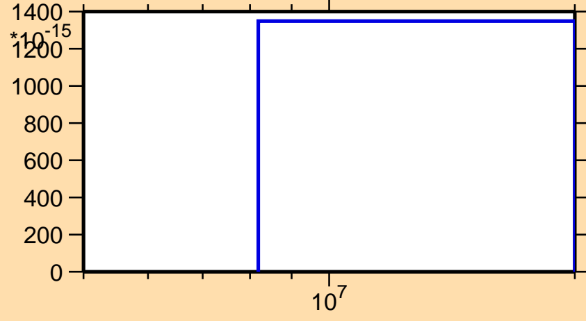
\sigma vs. E for ^{202}\text{Po}(n,nt)
