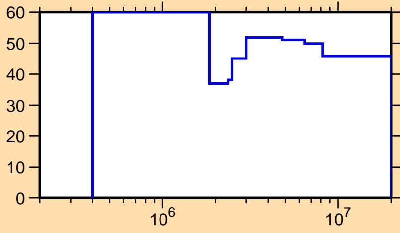
\Delta\sigma/\sigma vs. E for ^{202}\text{Po}(n,n_1)
