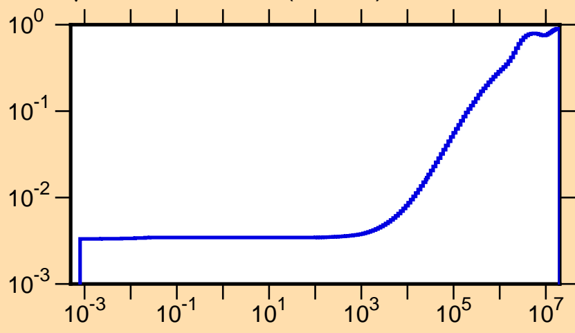
\mu vs. E for ^{203}\text{Po}(\text{mt251})
